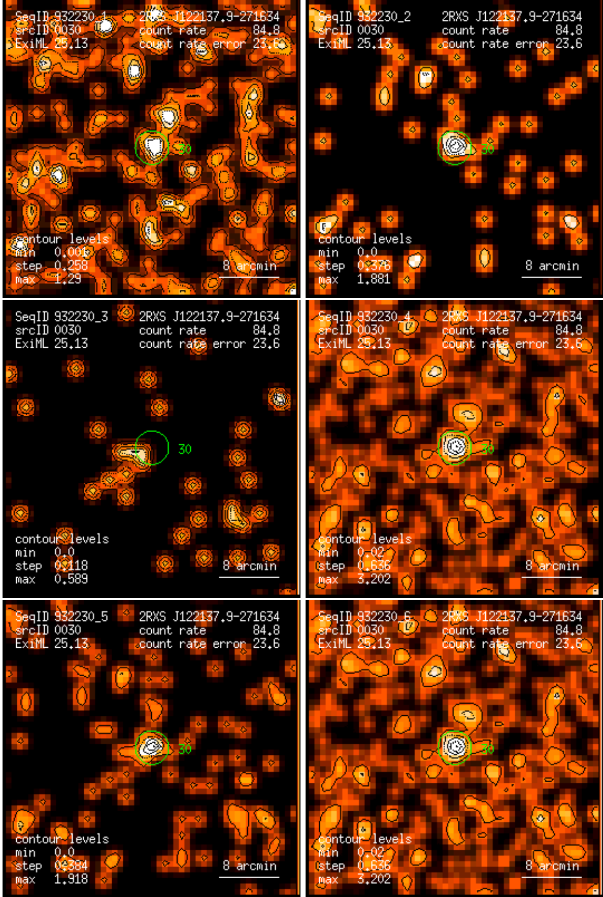
Figure 30: RASS 932230: detection 0030: band rate images, Gaussian filter: (1) PSPC channels 11 – 41, (2) 52 – 90, (3) 91 – 201, (4) 11 – 235, (5) 52 – 201, (6) 11 – 201. Broad band rates in counts/ks. Band rate contour levels in counts/ks/arcmin 2 .
