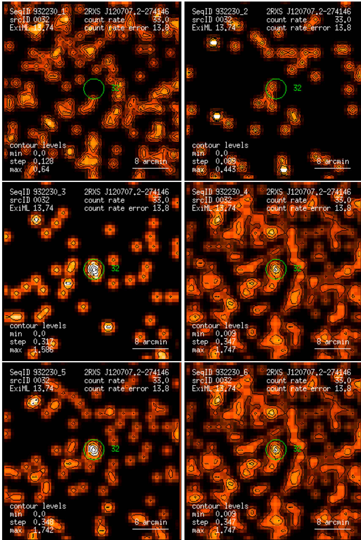
Figure 32: RASS 932230: detection 0032: band rate images, Gaussian filter: (1) PSPC channels 11 – 41, (2) 52 – 90, (3) 91 – 201, (4) 11 – 235, (5) 52 – 201, (6) 11 – 201. Broad band rates in counts/ks. Band rate contour levels in counts/ks/arcmin 2 .
