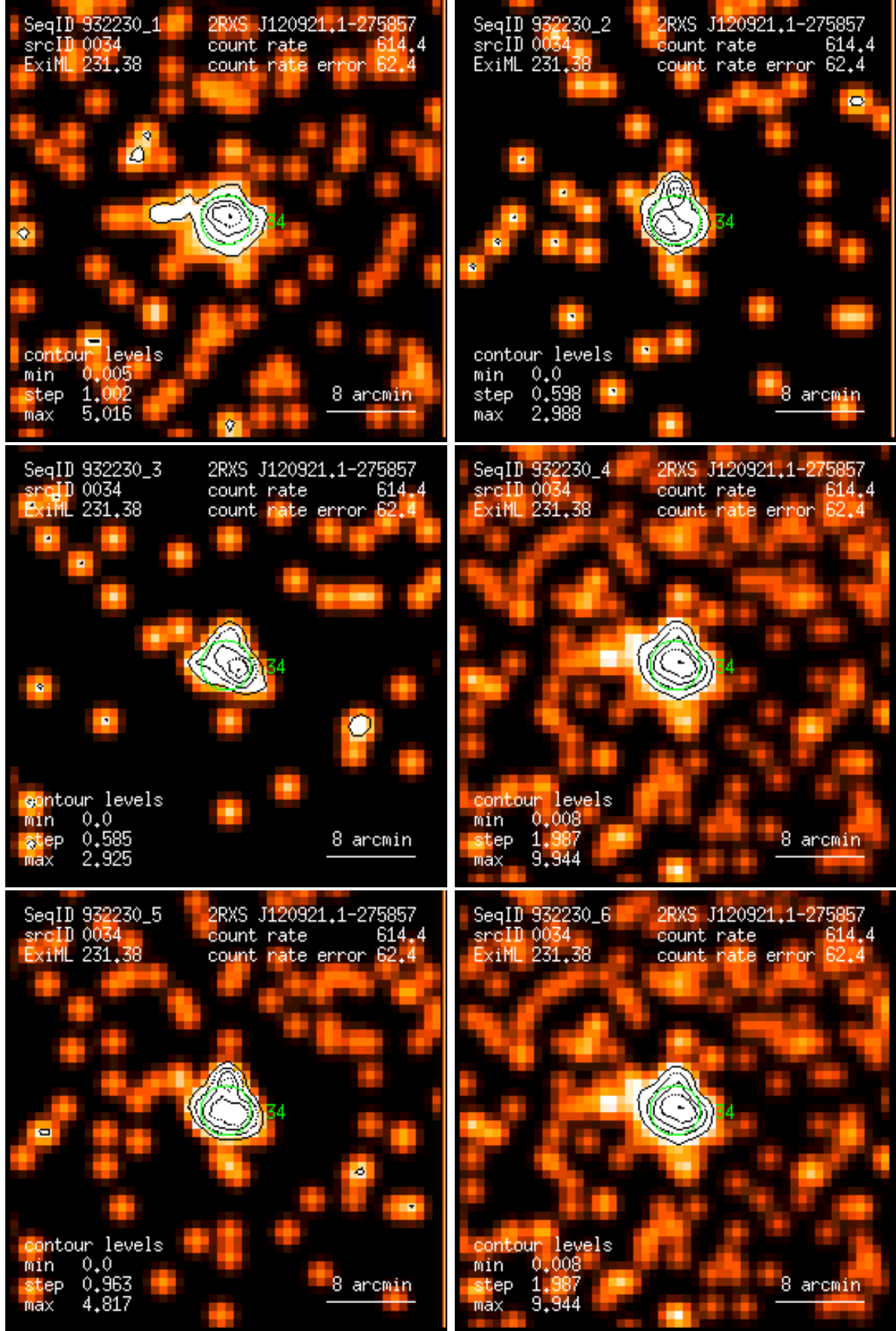
Figure 34: RASS 932230: detection 0034: band rate images, Gaussian filter: (1) PSPC channels 11 – 41, (2) 52 – 90, (3) 91 – 201, (4) 11 – 235, (5) 52 – 201, (6) 11 – 201. Broad band rates in counts/ks. Band rate contour levels in counts/ks/arcmin 2 .
