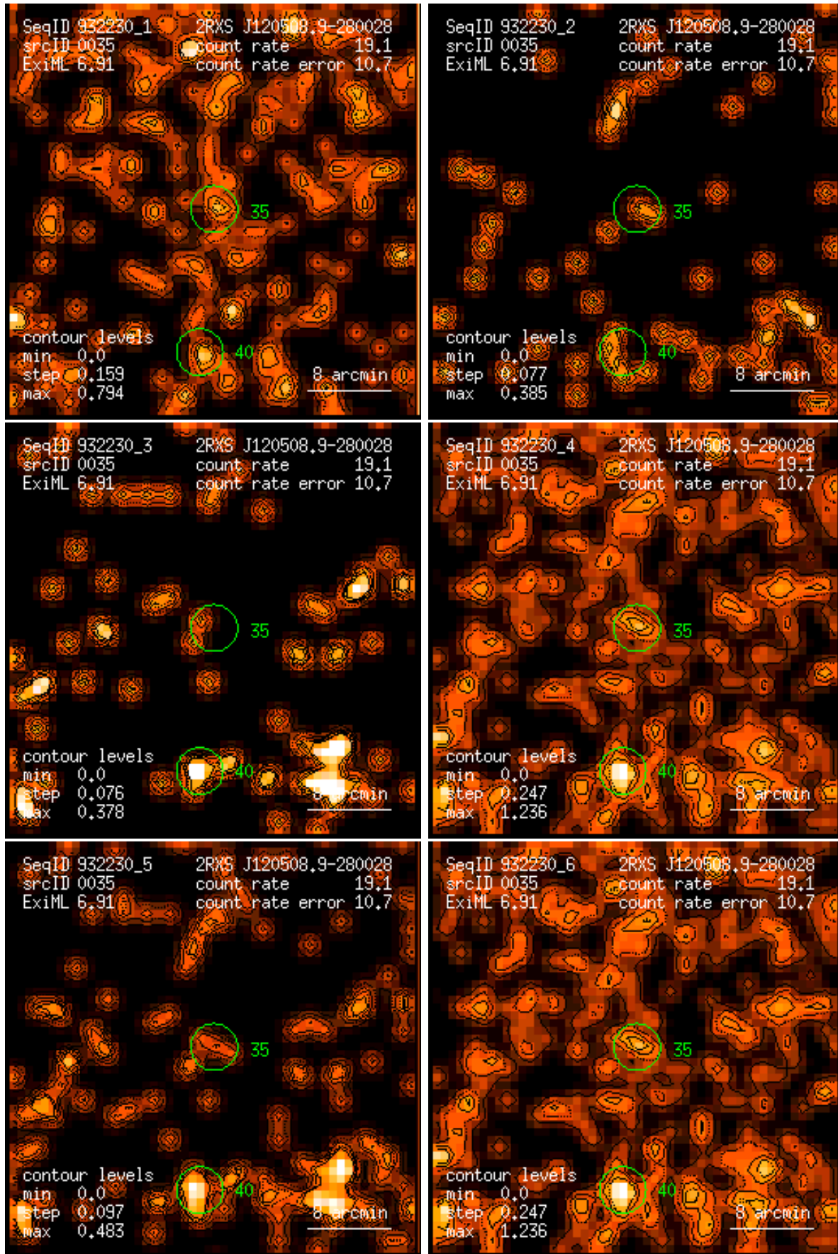
Figure 35: RASS 932230: detection 0035: band rate images, Gaussian filter: (1) PSPC channels 11 – 41, (2) 52 – 90, (3) 91 – 201, (4) 11 – 235, (5) 52 – 201, (6) 11 – 201. Broad band rates in counts/ks. Band rate contour levels in counts/ks/arcmin 2 .
