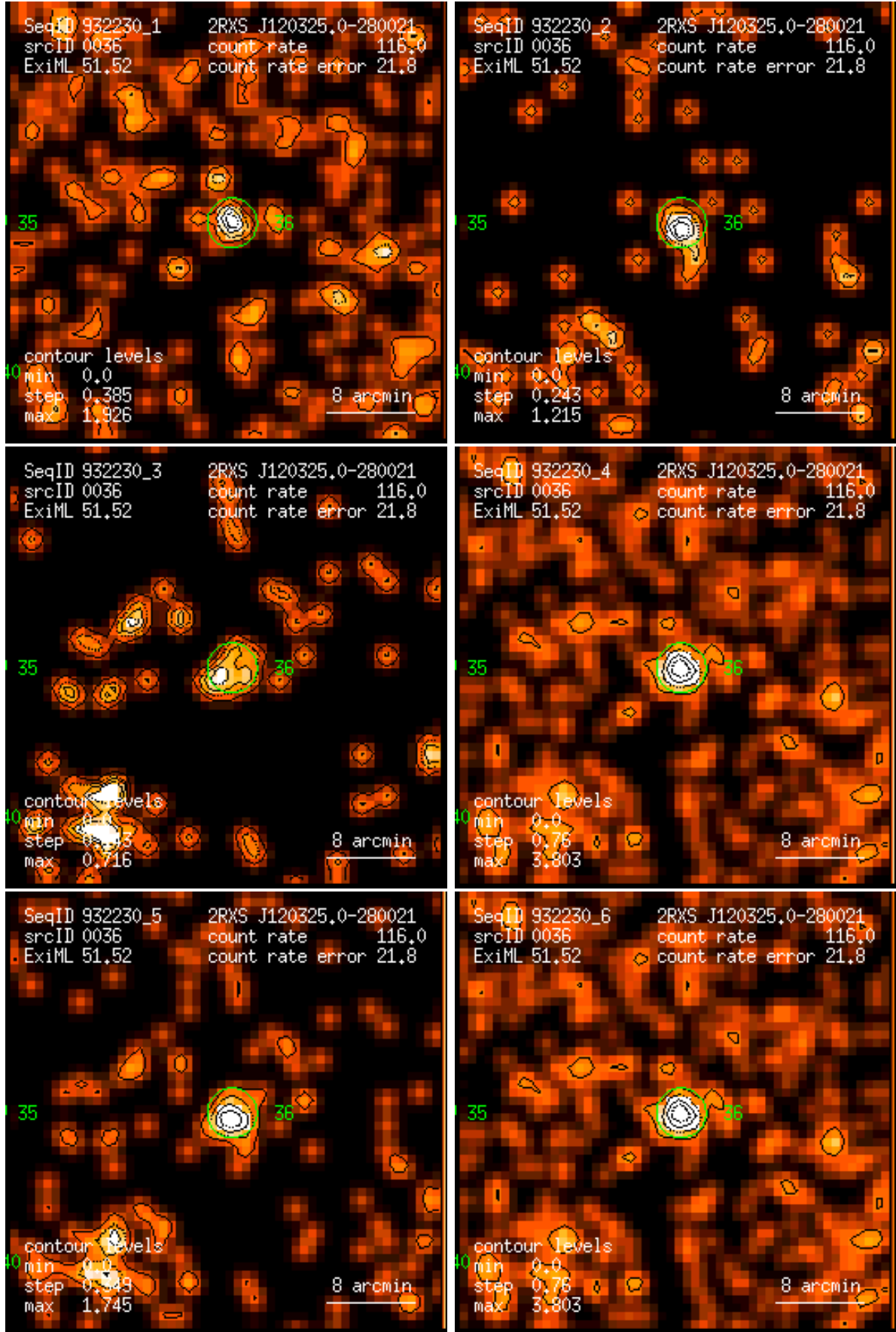
Figure 36: RASS 932230: detection 0036: band rate images, Gaussian filter: (1) PSPC channels 11 – 41, (2) 52 – 90, (3) 91 – 201, (4) 11 – 235, (5) 52 – 201, (6) 11 – 201. Broad band rates in counts/ks. Band rate contour levels in counts/ks/arcmin 2 .
