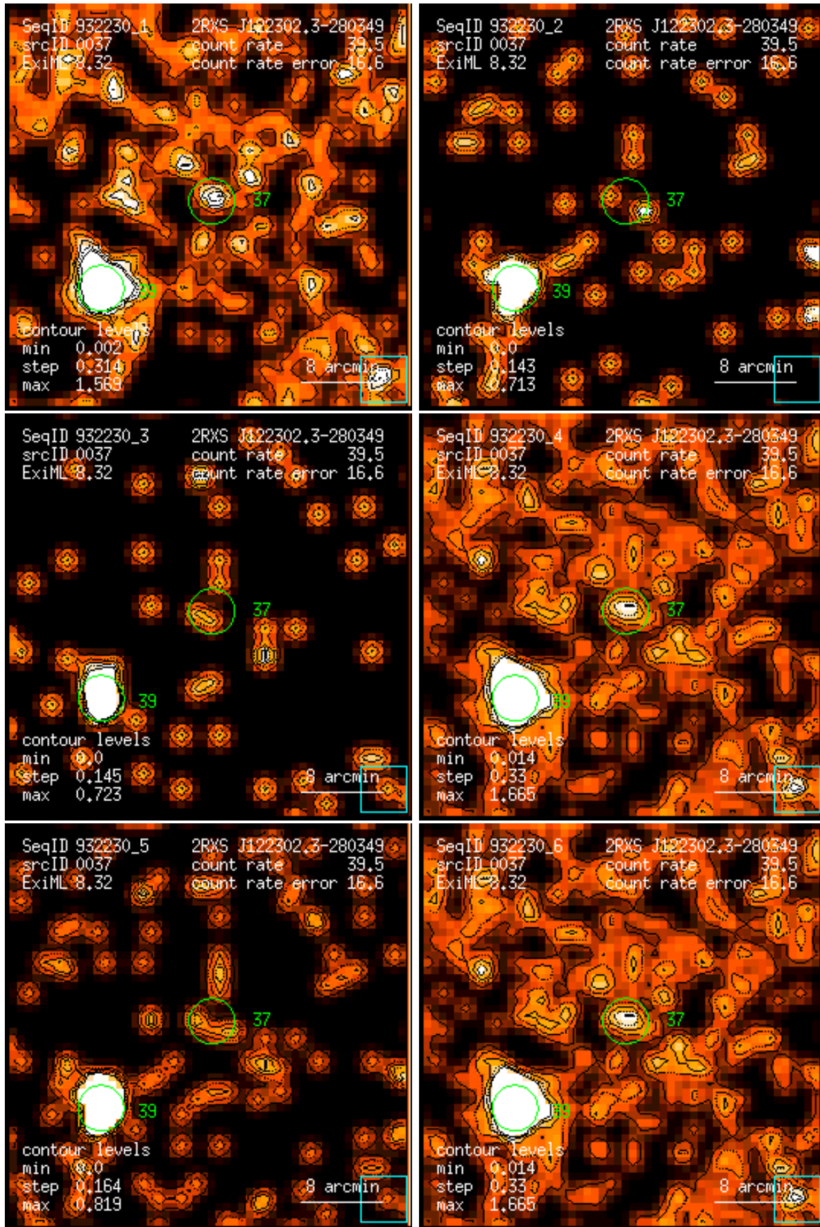
Figure 37: RASS 932230: detection 0037: band rate images, Gaussian filter: (1) PSPC channels 11 – 41, (2) 52 – 90, (3) 91 – 201, (4) 11 – 235, (5) 52 – 201, (6) 11 – 201. Broad band rates in counts/ks. Band rate contour levels in counts/ks/arcmin 2 .
