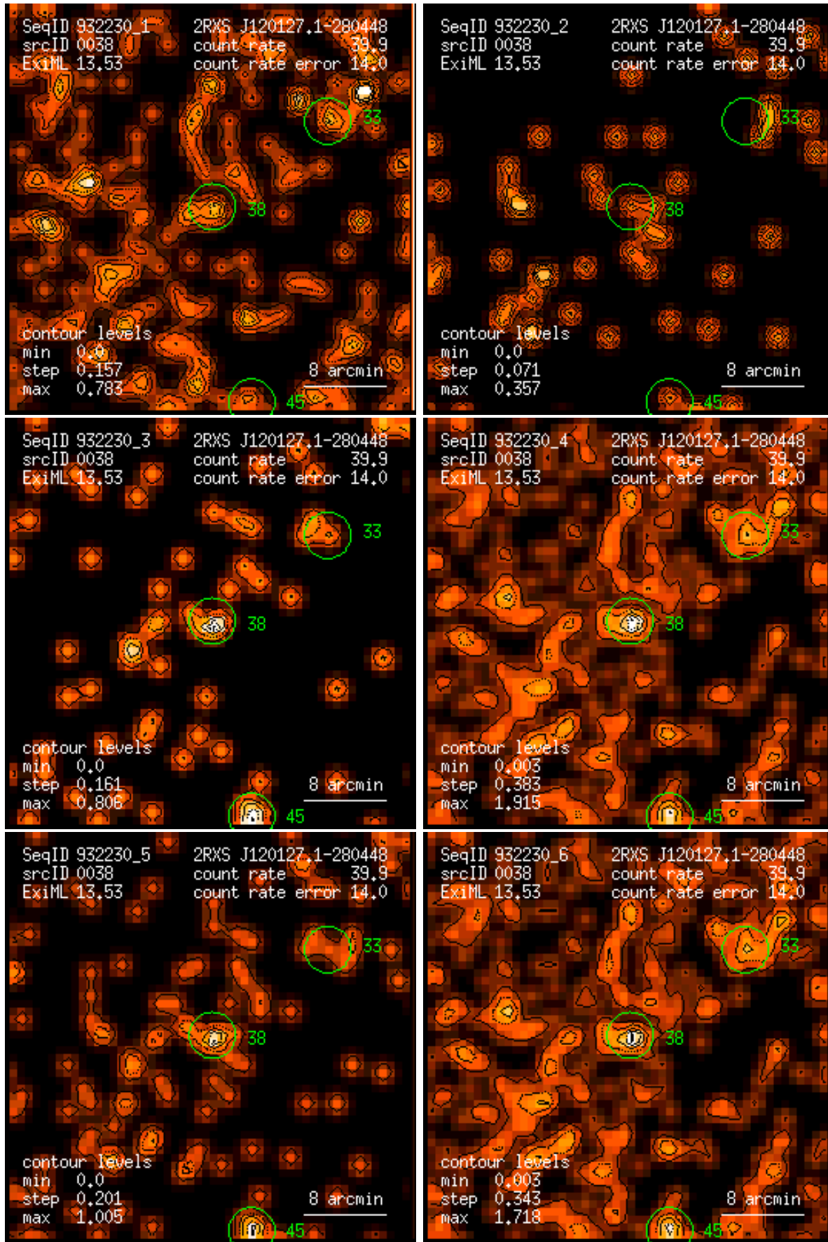
Figure 38: RASS 932230: detection 0038: band rate images, Gaussian filter: (1) PSPC channels 11 – 41, (2) 52 – 90, (3) 91 – 201, (4) 11 – 235, (5) 52 – 201, (6) 11 – 201. Broad band rates in counts/ks. Band rate contour levels in counts/ks/arcmin 2 .
