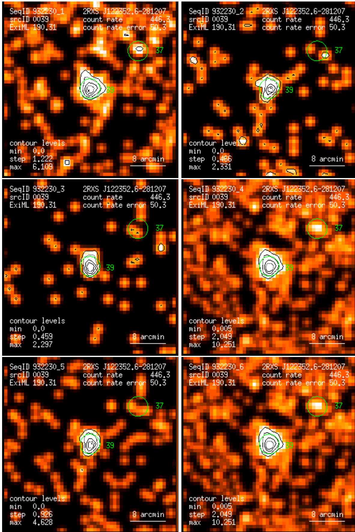
Figure 39: RASS 932230: detection 0039: band rate images, Gaussian filter: (1) PSPC channels 11 – 41, (2) 52 – 90, (3) 91 – 201, (4) 11 – 235, (5) 52 – 201, (6) 11 – 201. Broad band rates in counts/ks. Band rate contour levels in counts/ks/arcmin 2 .
