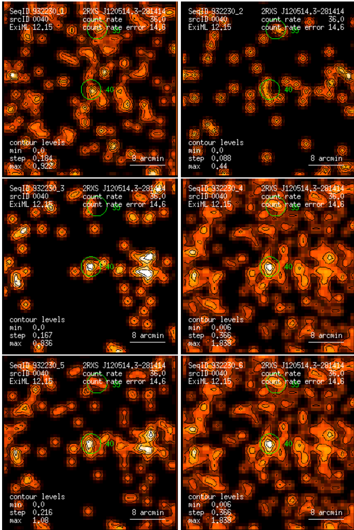
Figure 40: RASS 932230: detection 0040: band rate images, Gaussian filter: (1) PSPC channels 11 – 41, (2) 52 – 90, (3) 91 – 201, (4) 11 – 235, (5) 52 – 201, (6) 11 – 201. Broad band rates in counts/ks. Band rate contour levels in counts/ks/arcmin 2 .
