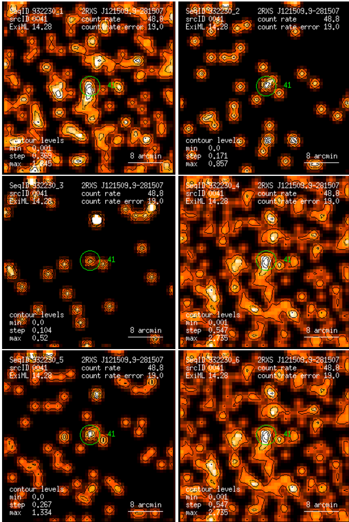
Figure 41: RASS 932230: detection 0041: band rate images, Gaussian filter: (1) PSPC channels 11 – 41, (2) 52 – 90, (3) 91 – 201, (4) 11 – 235, (5) 52 – 201, (6) 11 – 201. Broad band rates in counts/ks. Band rate contour levels in counts/ks/arcmin 2 .
