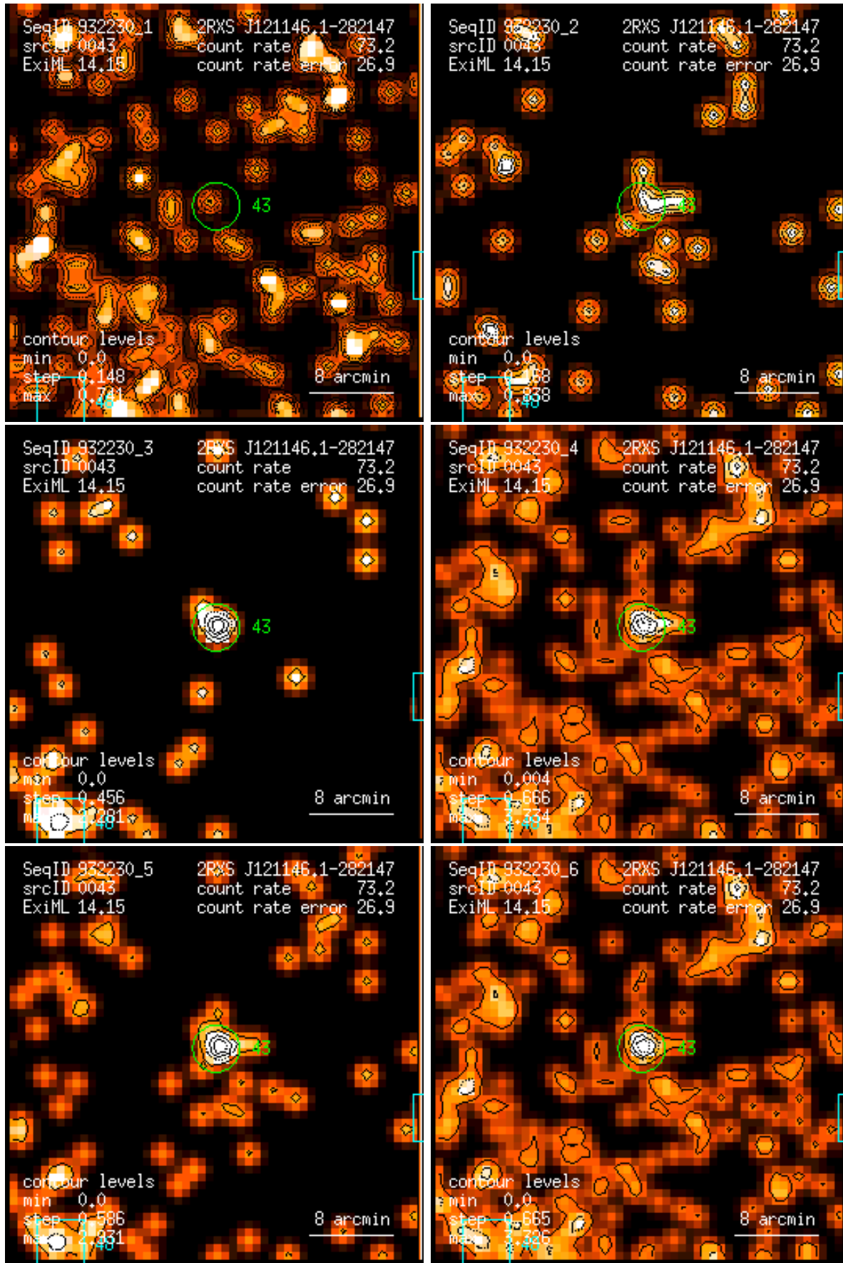
Figure 43: RASS 932230: detection 0043: band rate images, Gaussian filter: (1) PSPC channels 11 – 41, (2) 52 – 90, (3) 91 – 201, (4) 11 – 235, (5) 52 – 201, (6) 11 – 201. Broad band rates in counts/ks. Band rate contour levels in counts/ks/arcmin 2 .
