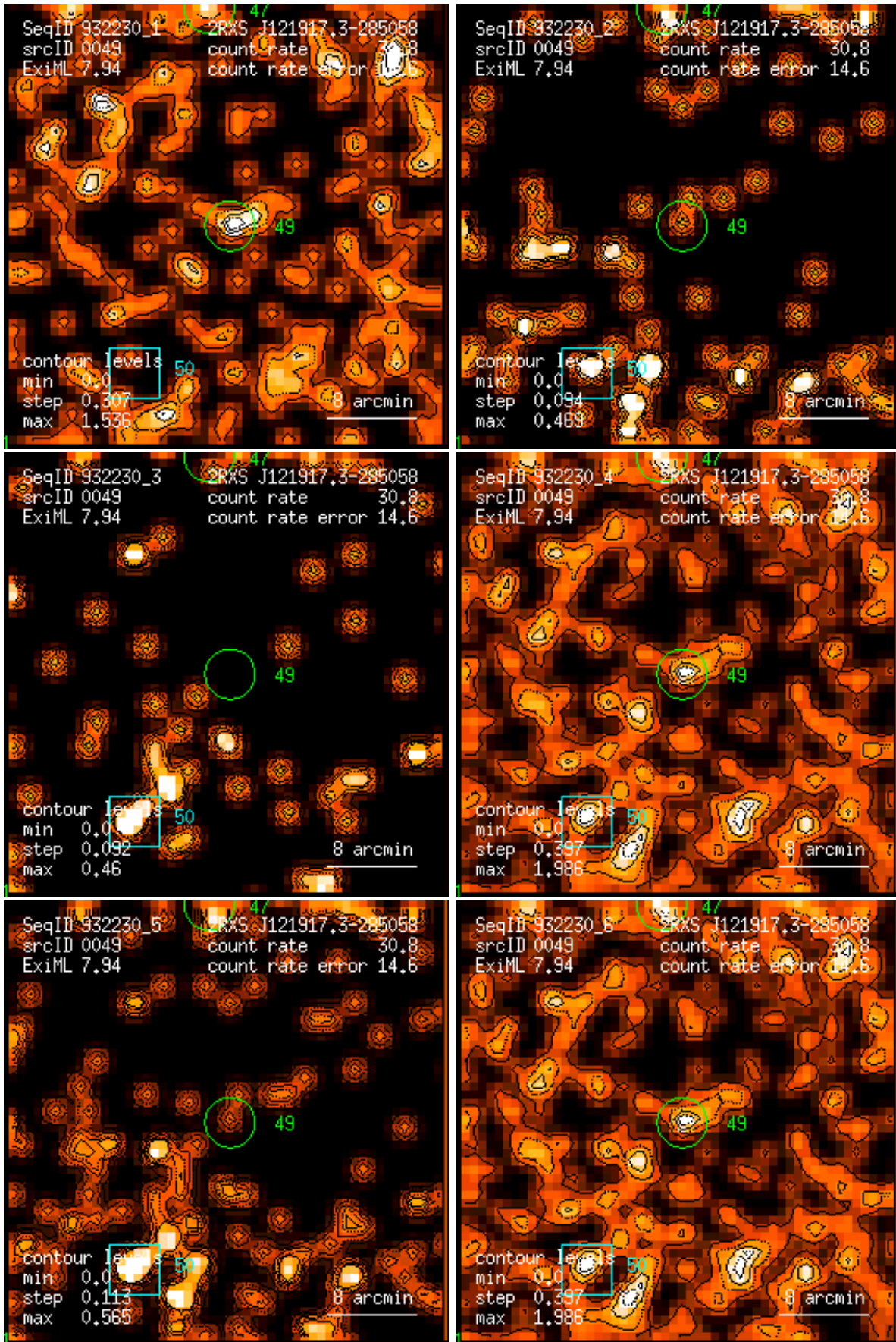
Figure 49: RASS 932230: detection 0049: band rate images, Gaussian filter: (1) PSPC channels 11 – 41, (2) 52 – 90, (3) 91 – 201, (4) 11 – 235, (5) 52 – 201, (6) 11 – 201. Broad band rates in counts/ks. Band rate contour levels in counts/ks/arcmin 2 .
