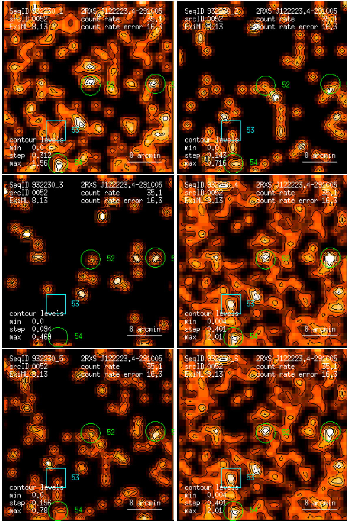
Figure 52: RASS 932230: detection 0052: band rate images, Gaussian filter: (1) PSPC channels 11 – 41, (2) 52 – 90, (3) 91 – 201, (4) 11 – 235, (5) 52 – 201, (6) 11 – 201. Broad band rates in counts/ks. Band rate contour levels in counts/ks/arcmin 2 .
