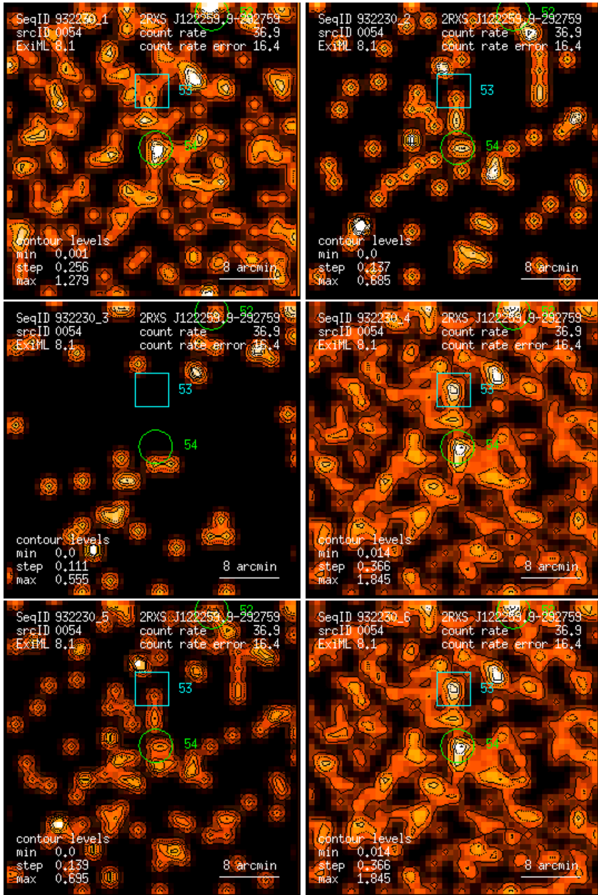
Figure 54: RASS 932230: detection 0054: band rate images, Gaussian filter: (1) PSPC channels 11 – 41, (2) 52 – 90, (3) 91 – 201, (4) 11 – 235, (5) 52 – 201, (6) 11 – 201. Broad band rates in counts/ks. Band rate contour levels in counts/ks/arcmin 2 .
