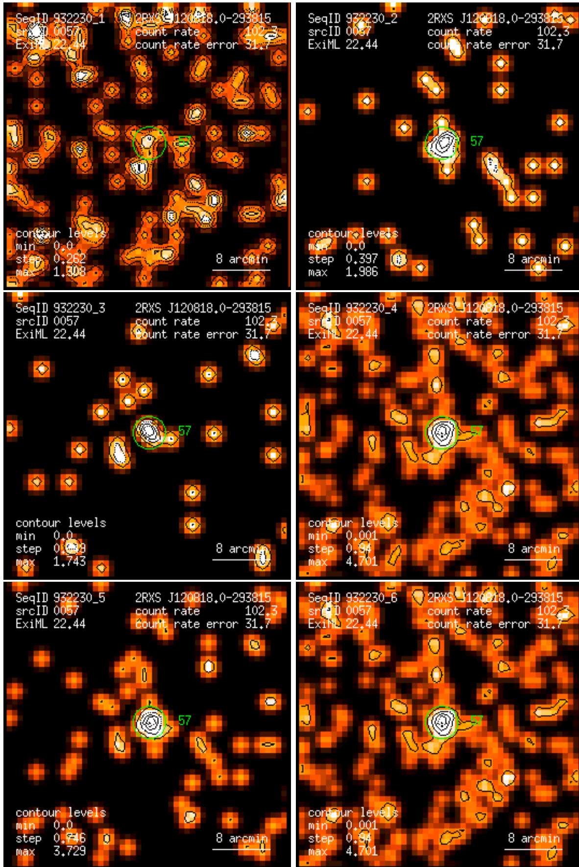
Figure 57: RASS 932230: detection 0057: band rate images, Gaussian filter: (1) PSPC channels 11 – 41, (2) 52 – 90, (3) 91 – 201, (4) 11 – 235, (5) 52 – 201, (6) 11 – 201. Broad band rates in counts/ks. Band rate contour levels in counts/ks/arcmin 2 .
