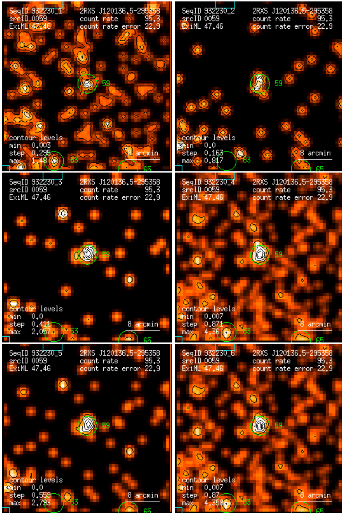
Figure 59: RASS 932230: detection 0059: band rate images, Gaussian filter: (1) PSPC channels 11 – 41, (2) 52 – 90, (3) 91 – 201, (4) 11 – 235, (5) 52 – 201, (6) 11 – 201. Broad band rates in counts/ks. Band rate contour levels in counts/ks/arcmin 2 .
