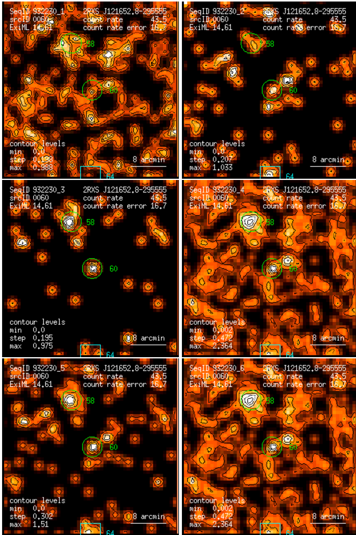
Figure 60: RASS 932230: detection 0060: band rate images, Gaussian filter: (1) PSPC channels 11 – 41, (2) 52 – 90, (3) 91 – 201, (4) 11 – 235, (5) 52 – 201, (6) 11 – 201. Broad band rates in counts/ks. Band rate contour levels in counts/ks/arcmin 2 .
