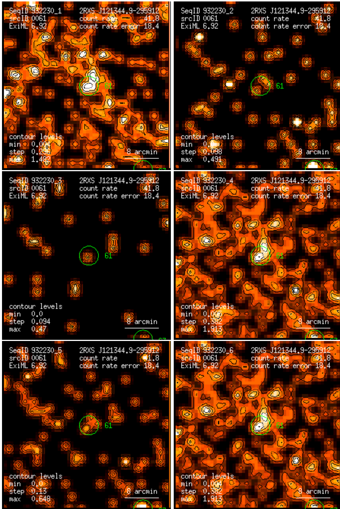
Figure 61: RASS 932230: detection 0061: band rate images, Gaussian filter: (1) PSPC channels 11 – 41, (2) 52 – 90, (3) 91 – 201, (4) 11 – 235, (5) 52 – 201, (6) 11 – 201. Broad band rates in counts/ks. Band rate contour levels in counts/ks/arcmin 2 .
