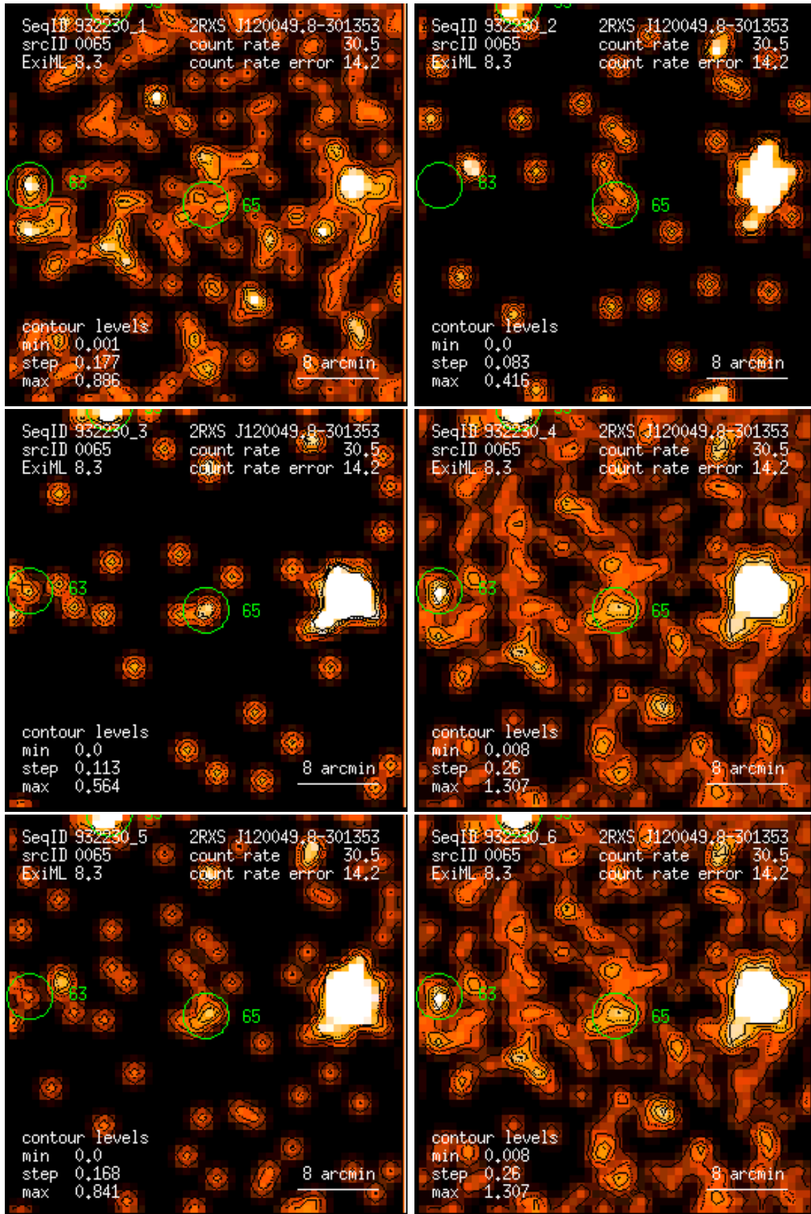
Figure 65: RASS 932230: detection 0065: band rate images, Gaussian filter: (1) PSPC channels 11 – 41, (2) 52 – 90, (3) 91 – 201, (4) 11 – 235, (5) 52 – 201, (6) 11 – 201. Broad band rates in counts/ks. Band rate contour levels in counts/ks/arcmin 2 .
