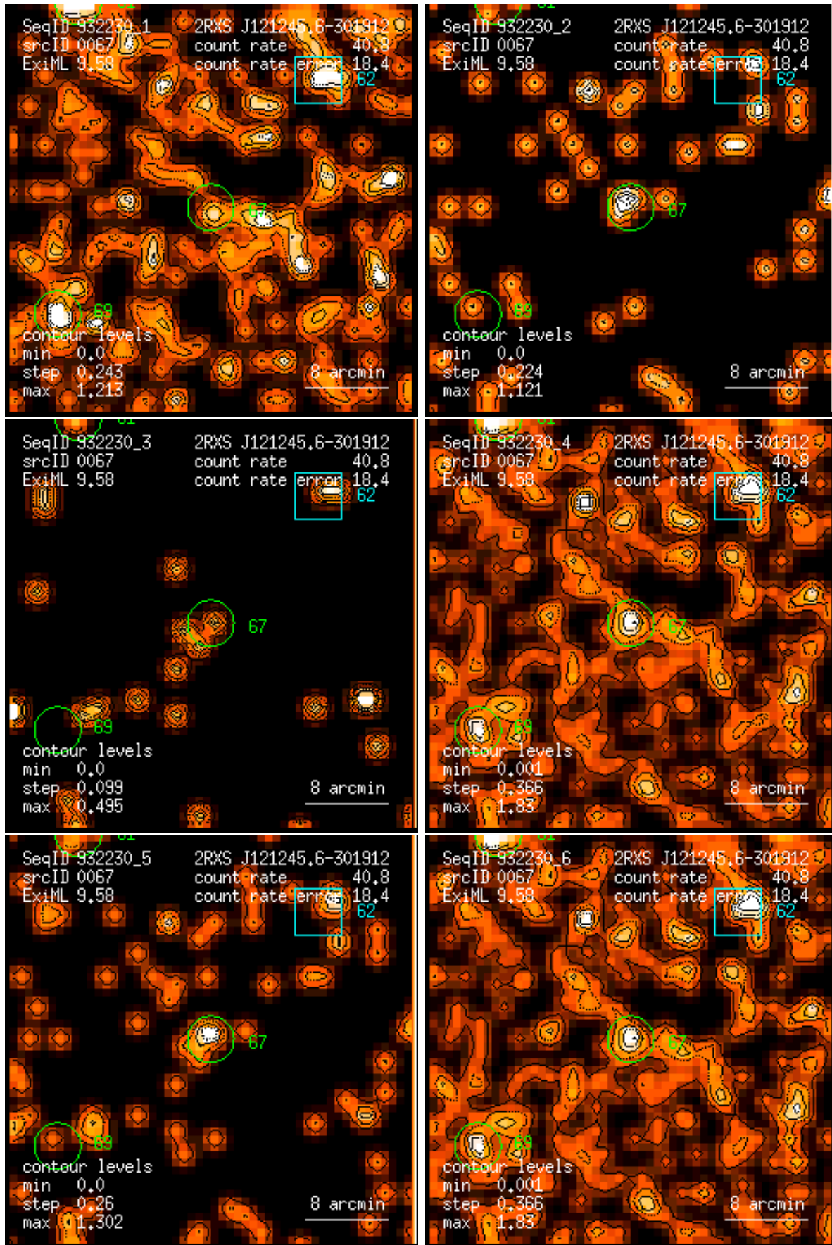
Figure 67: RASS 932230: detection 0067: band rate images, Gaussian filter: (1) PSPC channels 11 – 41, (2) 52 – 90, (3) 91 – 201, (4) 11 – 235, (5) 52 – 201, (6) 11 – 201. Broad band rates in counts/ks. Band rate contour levels in counts/ks/arcmin 2 .
