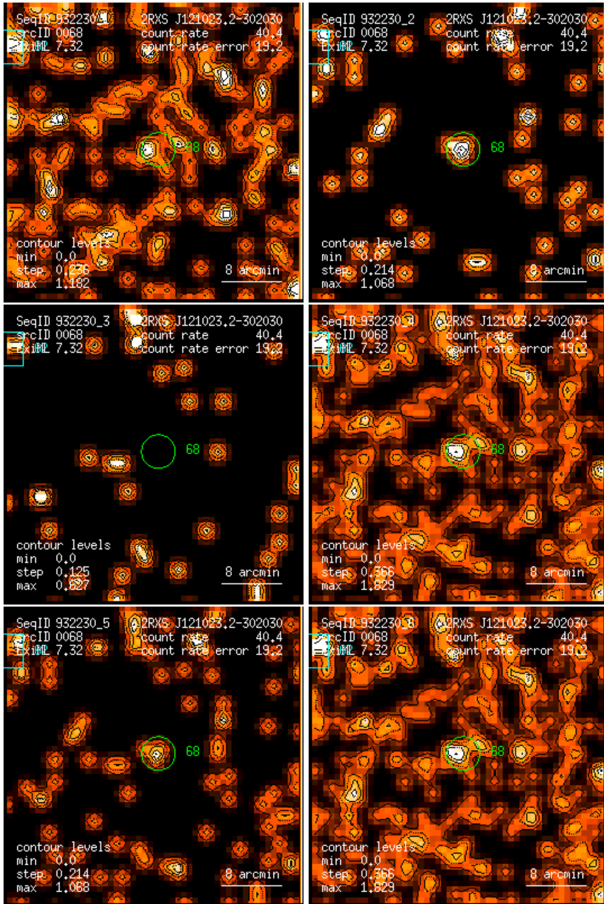
Figure 68: RASS 932230: detection 0068: band rate images, Gaussian filter: (1) PSPC channels 11 – 41, (2) 52 – 90, (3) 91 – 201, (4) 11 – 235, (5) 52 – 201, (6) 11 – 201. Broad band rates in counts/ks. Band rate contour levels in counts/ks/arcmin 2 .
