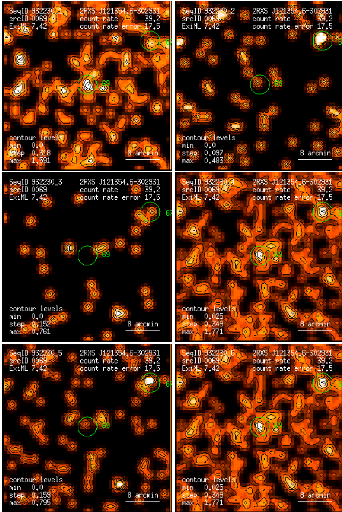
Figure 69: RASS 932230: detection 0069: band rate images, Gaussian filter: (1) PSPC channels 11 – 41, (2) 52 – 90, (3) 91 – 201, (4) 11 – 235, (5) 52 – 201, (6) 11 – 201. Broad band rates in counts/ks. Band rate contour levels in counts/ks/arcmin 2 .
