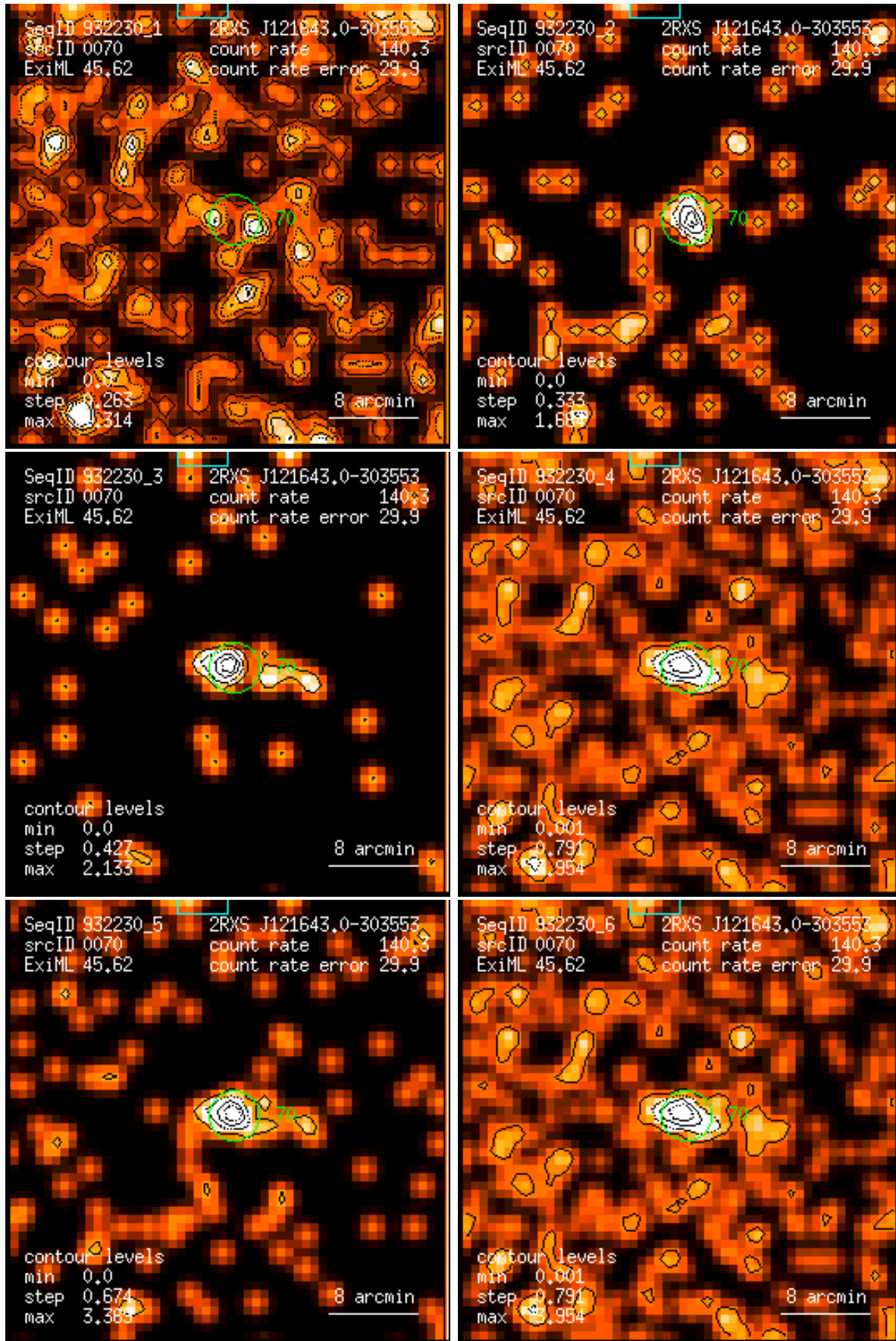
Figure 70: RASS 932230: detection 0070: band rate images, Gaussian filter: (1) PSPC channels 11 – 41, (2) 52 – 90, (3) 91 – 201, (4) 11 – 235, (5) 52 – 201, (6) 11 – 201. Broad band rates in counts/ks. Band rate contour levels in counts/ks/arcmin 2 .
