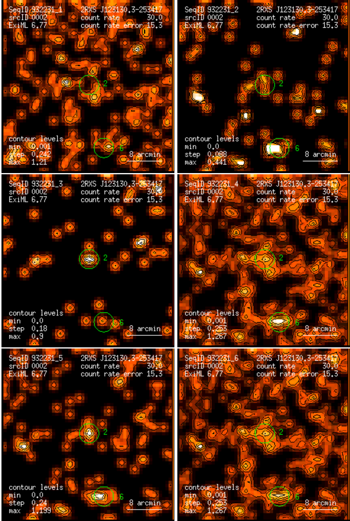
Figure 2: RASS 932231: detection 0002: band rate images, Gaussian filter: (1) PSPC channels 11 – 41, (2) 52 – 90, (3) 91 – 201, (4) 11 – 235, (5) 52 – 201, (6) 11 – 201. Broad band rates in counts/ks. Band rate contour levels in counts/ks/arcmin 2 .
