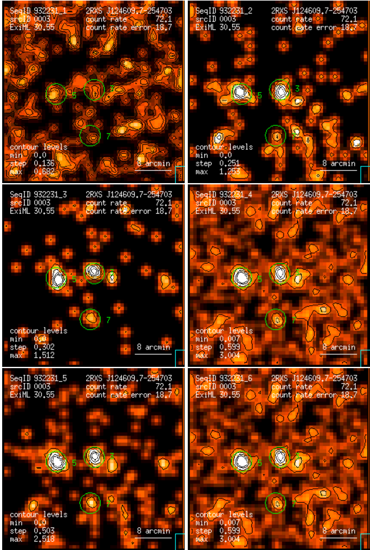
Figure 3: RASS 932231: detection 0003: band rate images, Gaussian filter: (1) PSPC channels 11 – 41, (2) 52 – 90, (3) 91 – 201, (4) 11 – 235, (5) 52 – 201, (6) 11 – 201. Broad band rates in counts/ks. Band rate contour levels in counts/ks/arcmin 2 .
