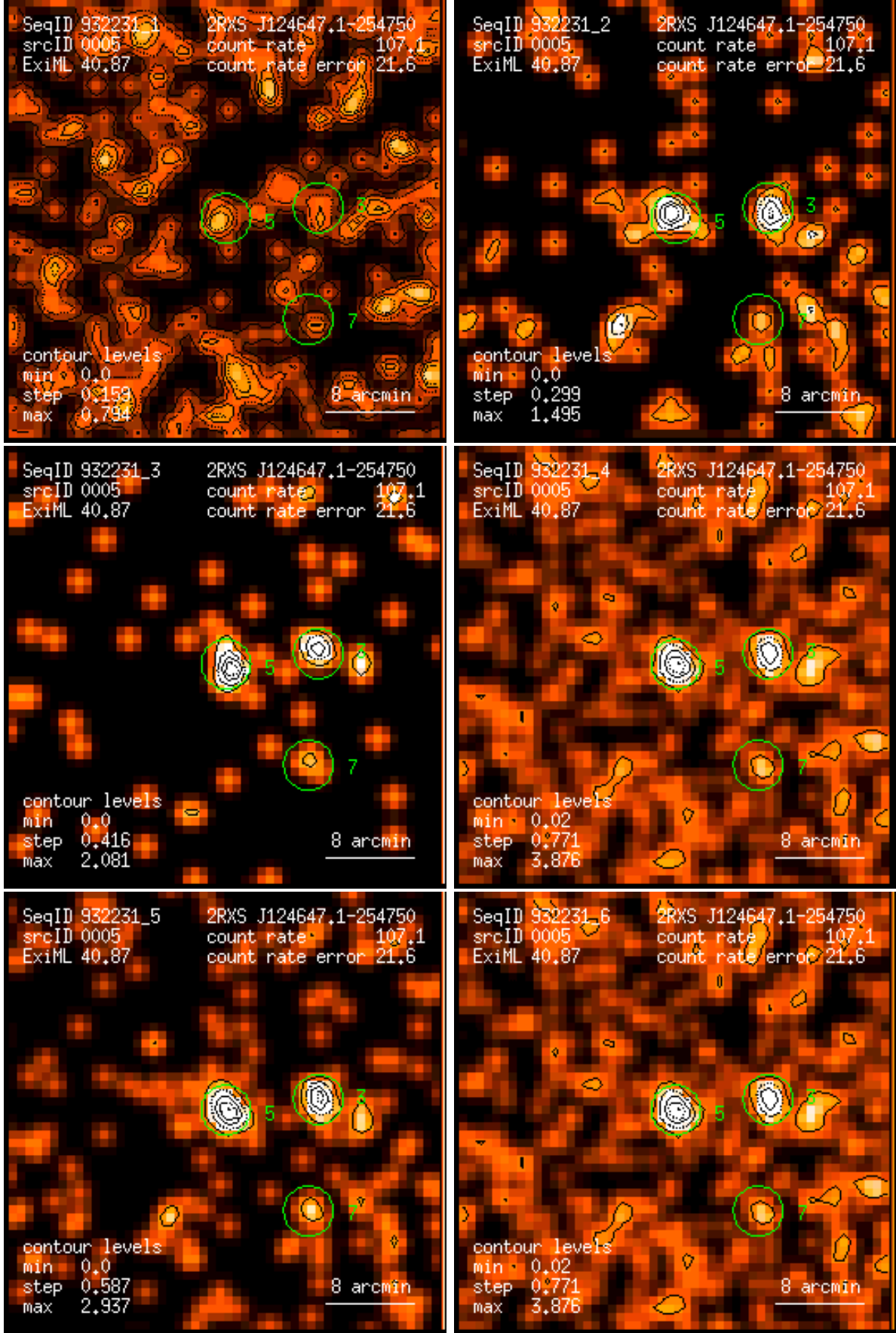
Figure 5: RASS 932231: detection 0005: band rate images, Gaussian filter: (1) PSPC channels 11 – 41, (2) 52 – 90, (3) 91 – 201, (4) 11 – 235, (5) 52 – 201, (6) 11 – 201. Broad band rates in counts/ks. Band rate contour levels in counts/ks/arcmin 2 .
