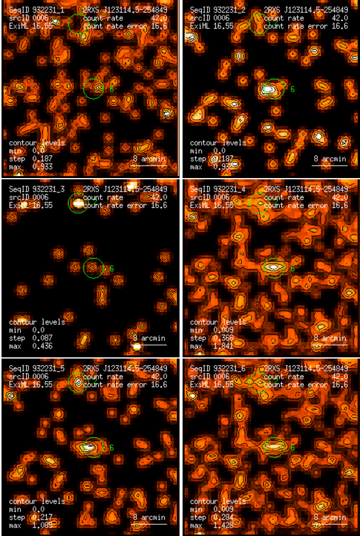
Figure 6: RASS 932231: detection 0006: band rate images, Gaussian filter: (1) PSPC channels 11 – 41, (2) 52 – 90, (3) 91 – 201, (4) 11 – 235, (5) 52 – 201, (6) 11 – 201. Broad band rates in counts/ks. Band rate contour levels in counts/ks/arcmin 2 .
