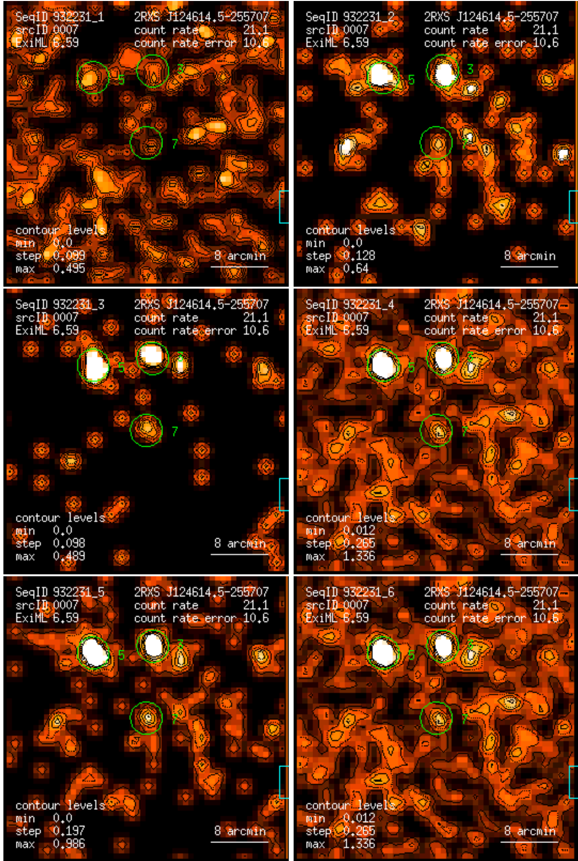
Figure 7: RASS 932231: detection 0007: band rate images, Gaussian filter: (1) PSPC channels 11 – 41, (2) 52 – 90, (3) 91 – 201, (4) 11 – 235, (5) 52 – 201, (6) 11 – 201. Broad band rates in counts/ks. Band rate contour levels in counts/ks/arcmin 2 .
