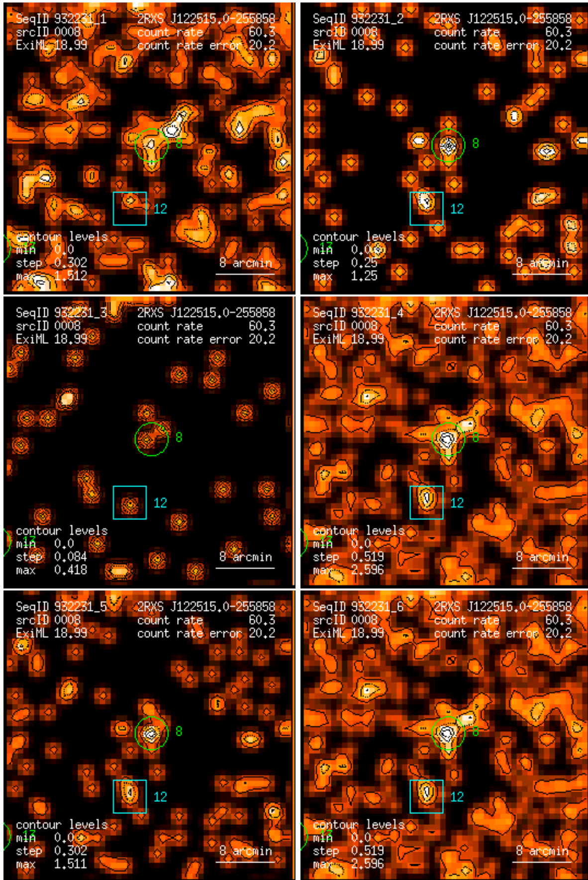
Figure 8: RASS 932231: detection 0008: band rate images, Gaussian filter: (1) PSPC channels 11 – 41, (2) 52 – 90, (3) 91 – 201, (4) 11 – 235, (5) 52 – 201, (6) 11 – 201. Broad band rates in counts/ks. Band rate contour levels in counts/ks/arcmin 2 .
