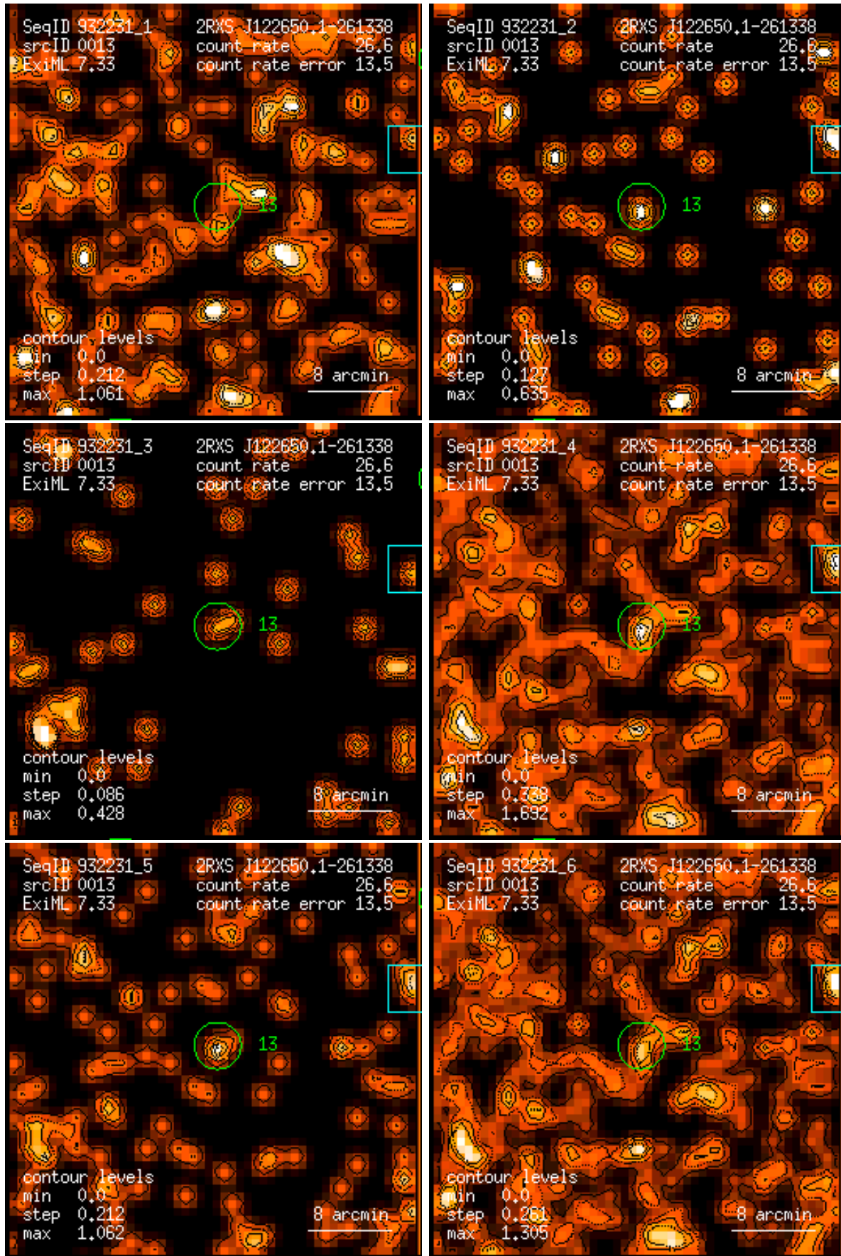
Figure 13: RASS 932231: detection 0013: band rate images, Gaussian filter: (1) PSPC channels 11 – 41, (2) 52 – 90, (3) 91 – 201, (4) 11 – 235, (5) 52 – 201, (6) 11 – 201. Broad band rates in counts/ks. Band rate contour levels in counts/ks/arcmin 2 .
