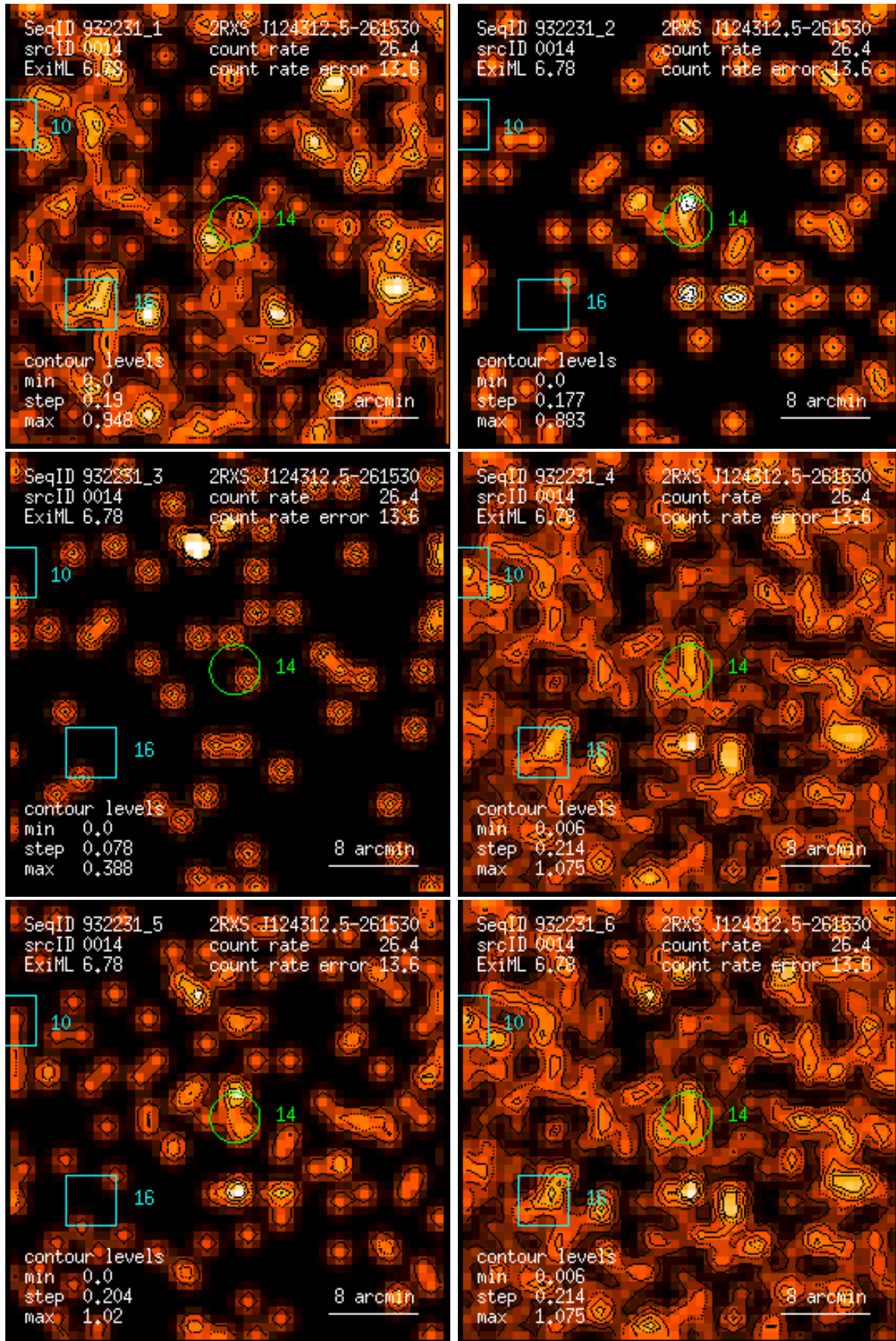
Figure 14: RASS 932231: detection 0014: band rate images, Gaussian filter: (1) PSPC channels 11 – 41, (2) 52 – 90, (3) 91 – 201, (4) 11 – 235, (5) 52 – 201, (6) 11 – 201. Broad band rates in counts/ks. Band rate contour levels in counts/ks/arcmin 2 .
