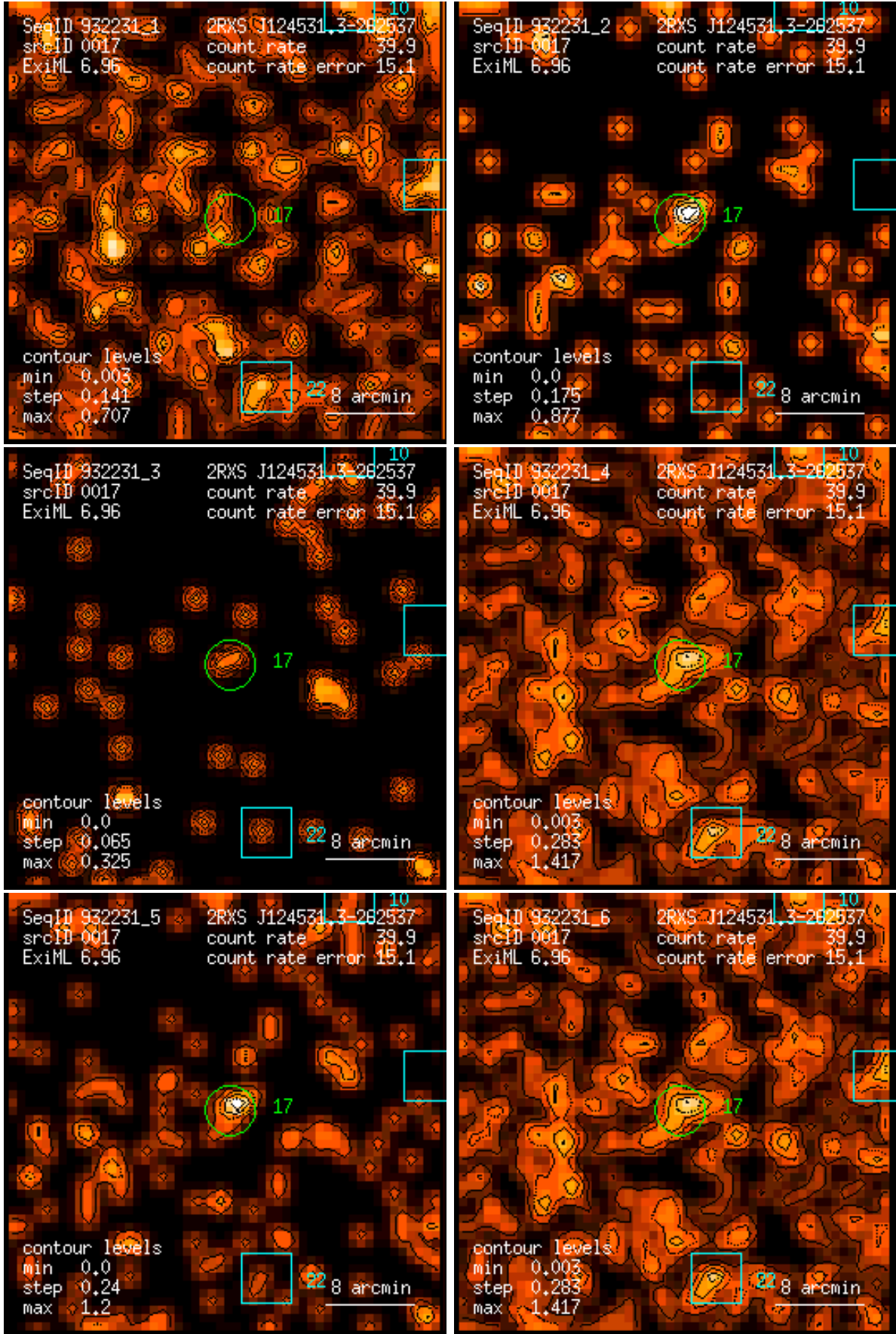
Figure 17: RASS 932231: detection 0017: band rate images, Gaussian filter: (1) PSPC channels 11 – 41, (2) 52 – 90, (3) 91 – 201, (4) 11 – 235, (5) 52 – 201, (6) 11 – 201. Broad band rates in counts/ks. Band rate contour levels in counts/ks/arcmin 2 .
