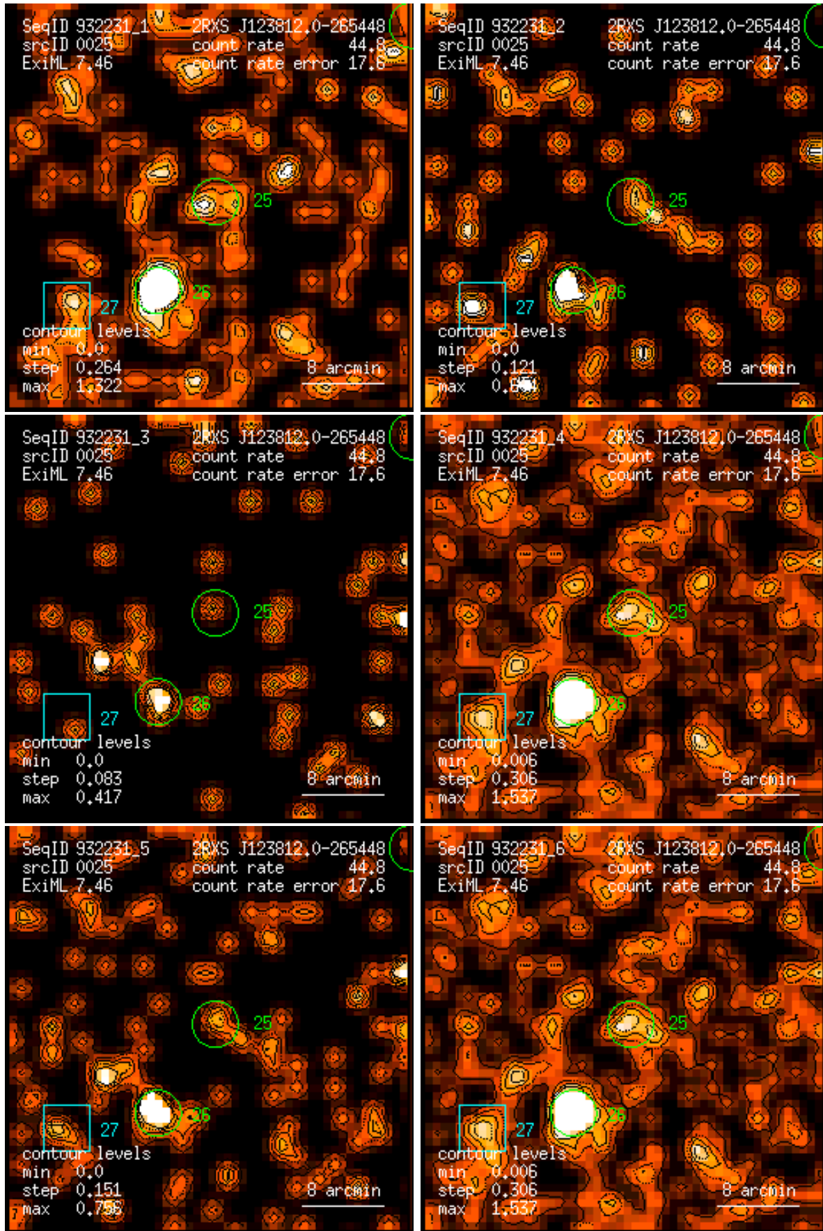
Figure 25: RASS 932231: detection 0025: band rate images, Gaussian filter: (1) PSPC channels 11 – 41, (2) 52 – 90, (3) 91 – 201, (4) 11 – 235, (5) 52 – 201, (6) 11 – 201. Broad band rates in counts/ks. Band rate contour levels in counts/ks/arcmin 2 .
