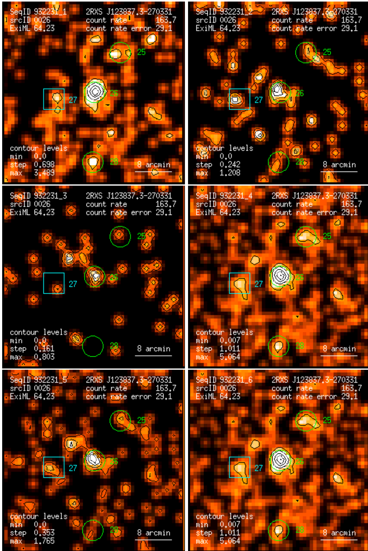
Figure 26: RASS 932231: detection 0026: band rate images, Gaussian filter: (1) PSPC channels 11 – 41, (2) 52 – 90, (3) 91 – 201, (4) 11 – 235, (5) 52 – 201, (6) 11 – 201. Broad band rates in counts/ks. Band rate contour levels in counts/ks/arcmin 2 .
