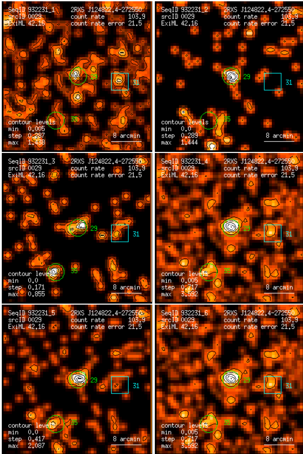
Figure 29: RASS 932231: detection 0029: band rate images, Gaussian filter: (1) PSPC channels 11 – 41, (2) 52 – 90, (3) 91 – 201, (4) 11 – 235, (5) 52 – 201, (6) 11 – 201. Broad band rates in counts/ks. Band rate contour levels in counts/ks/arcmin 2 .
