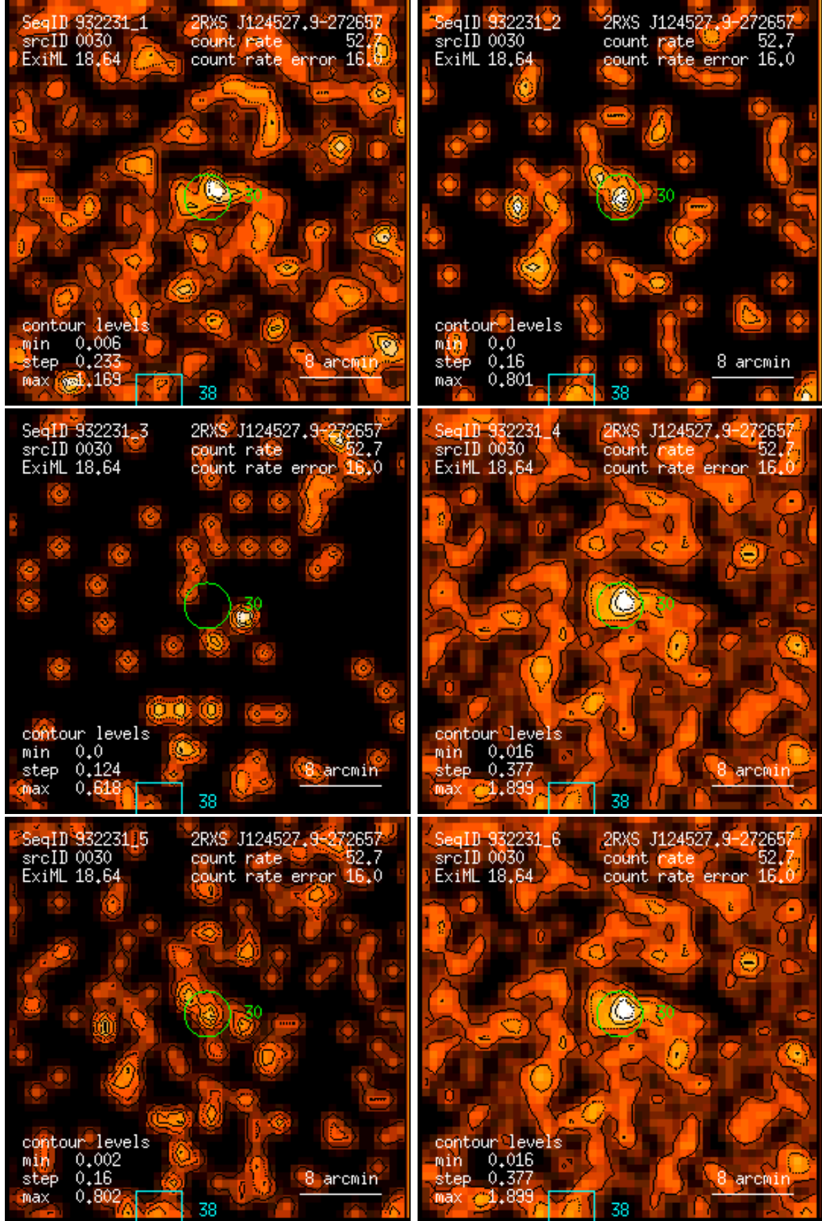
Figure 30: RASS 932231: detection 0030: band rate images, Gaussian filter: (1) PSPC channels 11 – 41, (2) 52 – 90, (3) 91 – 201, (4) 11 – 235, (5) 52 – 201, (6) 11 – 201. Broad band rates in counts/ks. Band rate contour levels in counts/ks/arcmin 2 .
