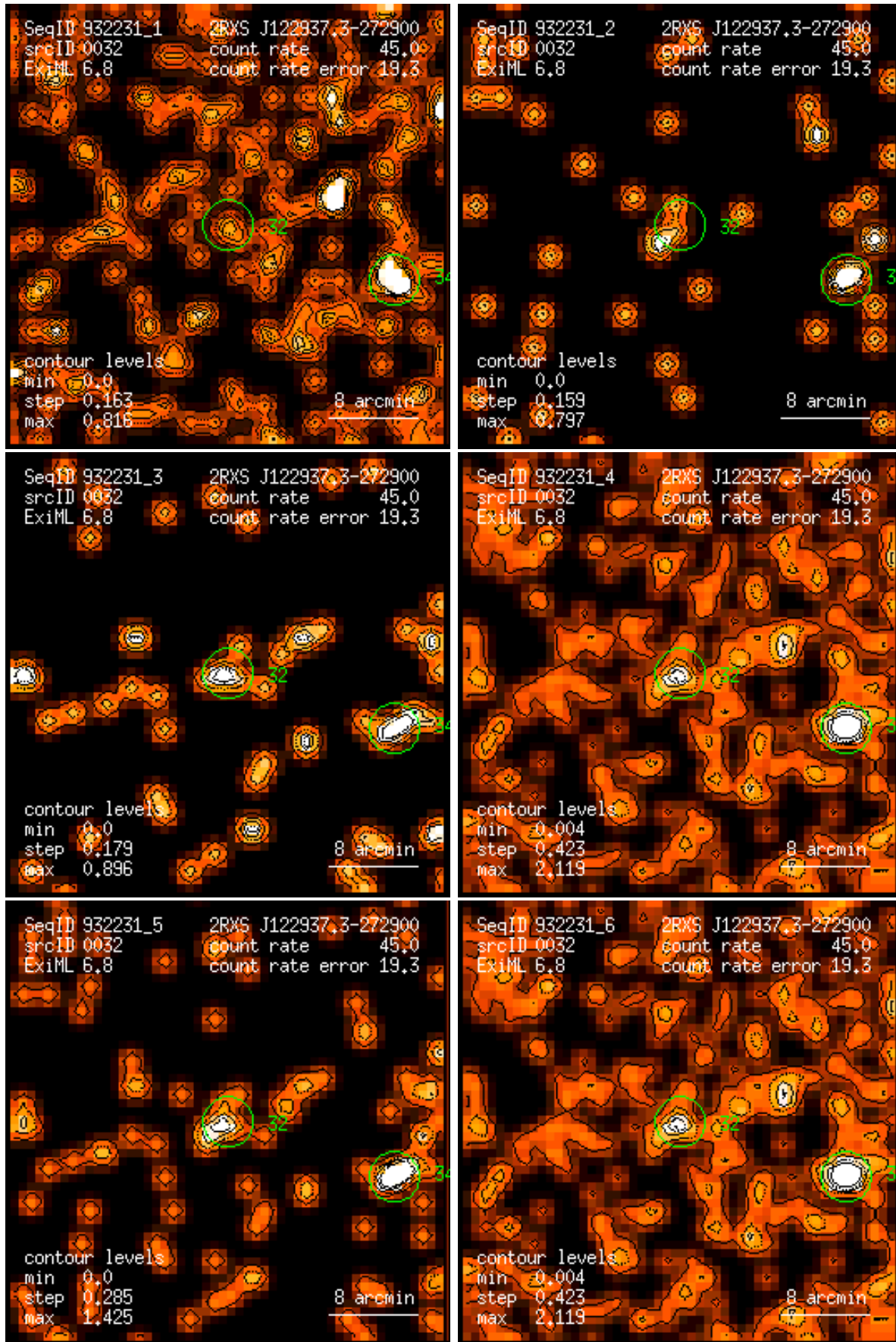
Figure 32: RASS 932231: detection 0032: band rate images, Gaussian filter: (1) PSPC channels 11 – 41, (2) 52 – 90, (3) 91 – 201, (4) 11 – 235, (5) 52 – 201, (6) 11 – 201. Broad band rates in counts/ks. Band rate contour levels in counts/ks/arcmin 2 .
