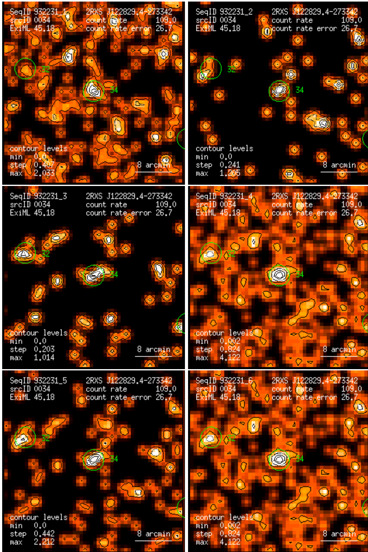
Figure 34: RASS 932231: detection 0034: band rate images, Gaussian filter: (1) PSPC channels 11 – 41, (2) 52 – 90, (3) 91 – 201, (4) 11 – 235, (5) 52 – 201, (6) 11 – 201. Broad band rates in counts/ks. Band rate contour levels in counts/ks/arcmin 2 .
