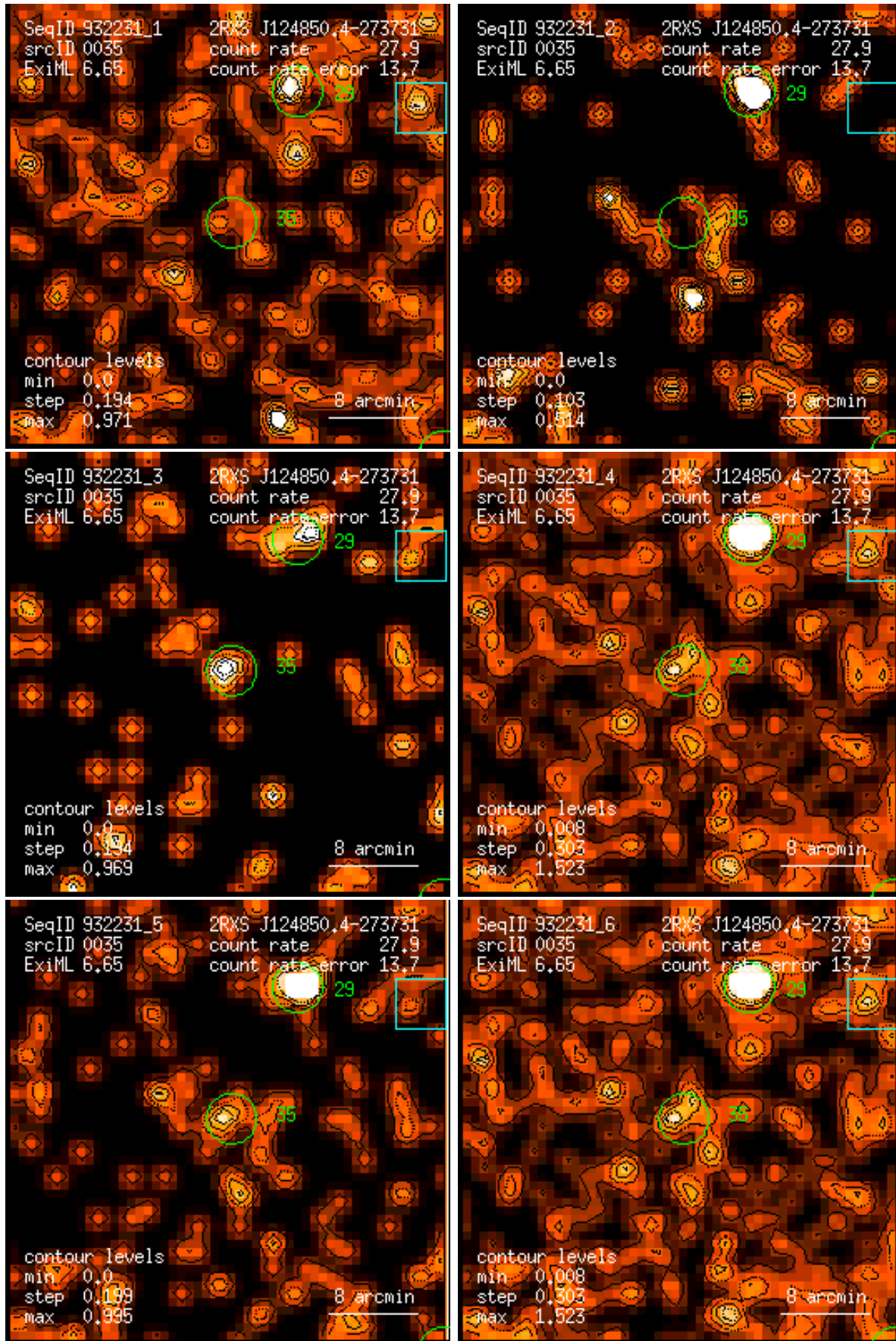
Figure 35: RASS 932231: detection 0035: band rate images, Gaussian filter: (1) PSPC channels 11 – 41, (2) 52 – 90, (3) 91 – 201, (4) 11 – 235, (5) 52 – 201, (6) 11 – 201. Broad band rates in counts/ks. Band rate contour levels in counts/ks/arcmin 2 .
