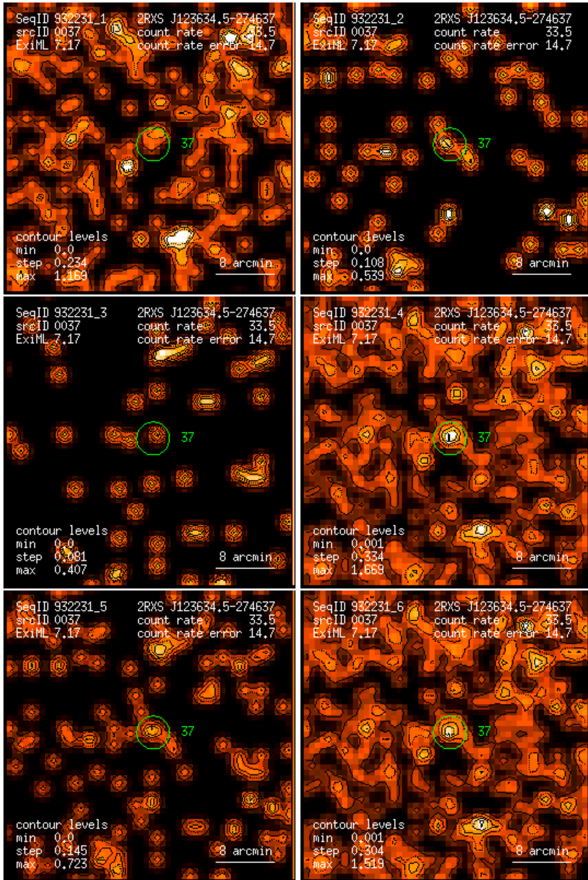
Figure 37: RASS 932231: detection 0037: band rate images, Gaussian filter: (1) PSPC channels 11 – 41, (2) 52 – 90, (3) 91 – 201, (4) 11 – 235, (5) 52 – 201, (6) 11 – 201. Broad band rates in counts/ks. Band rate contour levels in counts/ks/arcmin 2 .
