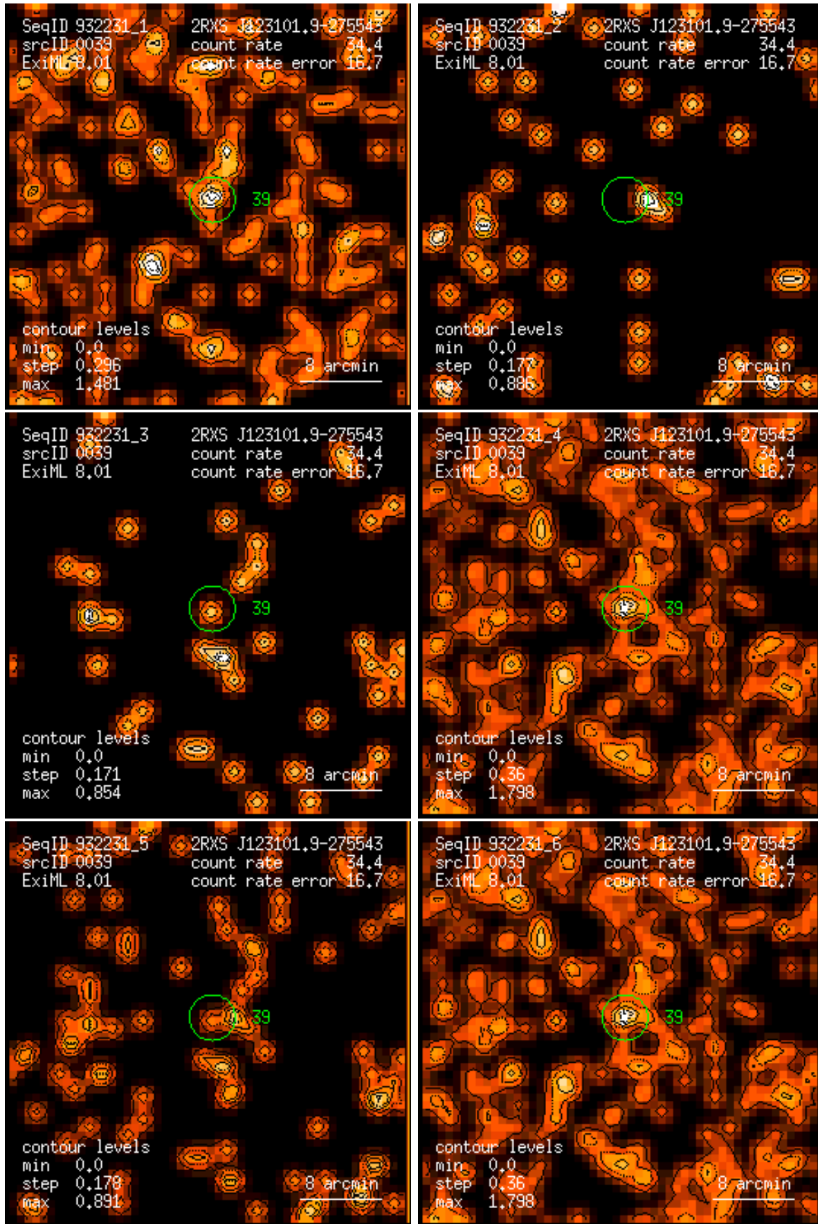
Figure 39: RASS 932231: detection 0039: band rate images, Gaussian filter: (1) PSPC channels 11 – 41, (2) 52 – 90, (3) 91 – 201, (4) 11 – 235, (5) 52 – 201, (6) 11 – 201. Broad band rates in counts/ks. Band rate contour levels in counts/ks/arcmin 2 .
