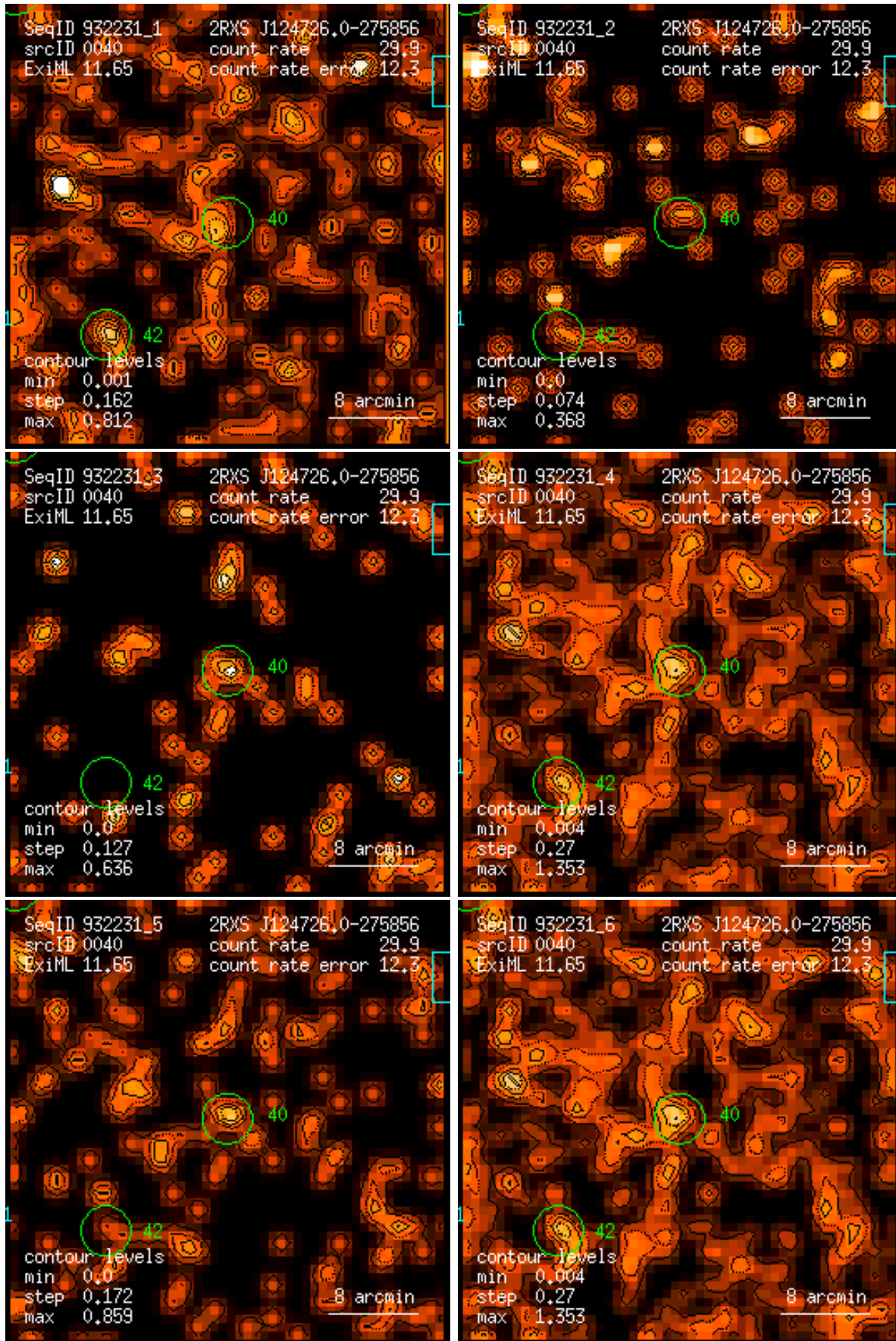
Figure 40: RASS 932231: detection 0040: band rate images, Gaussian filter: (1) PSPC channels 11 – 41, (2) 52 – 90, (3) 91 – 201, (4) 11 – 235, (5) 52 – 201, (6) 11 – 201. Broad band rates in counts/ks. Band rate contour levels in counts/ks/arcmin 2 .
