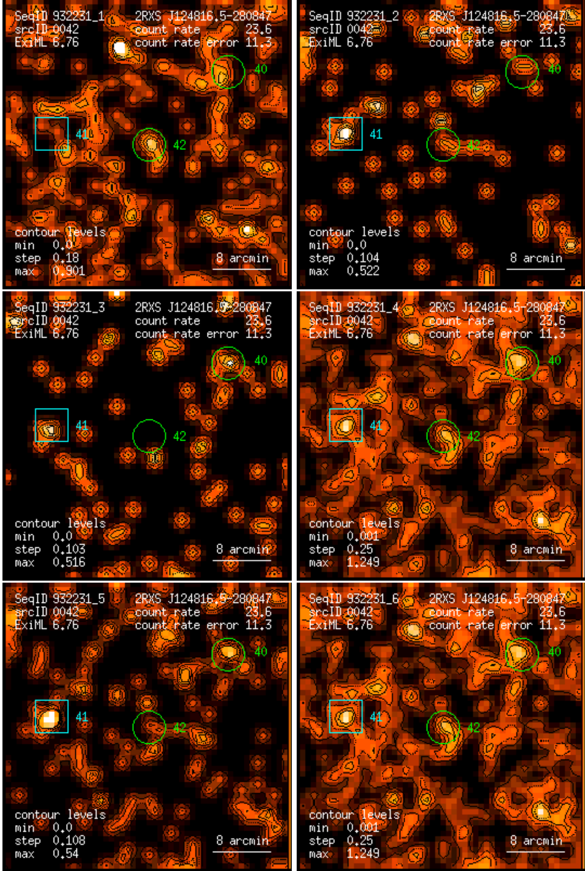
Figure 42: RASS 932231: detection 0042: band rate images, Gaussian filter: (1) PSPC channels 11 – 41, (2) 52 – 90, (3) 91 – 201, (4) 11 – 235, (5) 52 – 201, (6) 11 – 201. Broad band rates in counts/ks. Band rate contour levels in counts/ks/arcmin 2 .
