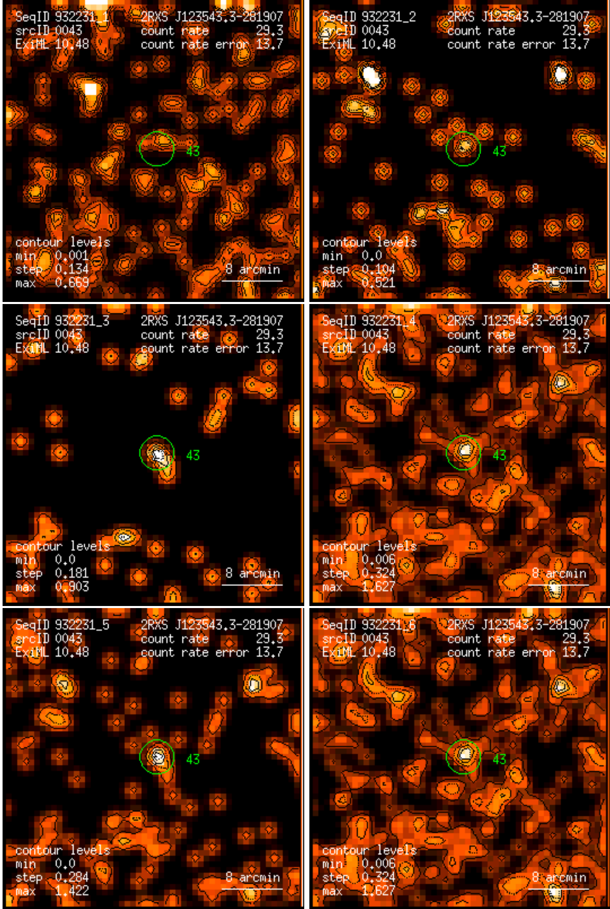
Figure 43: RASS 932231: detection 0043: band rate images, Gaussian filter: (1) PSPC channels 11 – 41, (2) 52 – 90, (3) 91 – 201, (4) 11 – 235, (5) 52 – 201, (6) 11 – 201. Broad band rates in counts/ks. Band rate contour levels in counts/ks/arcmin 2 .
