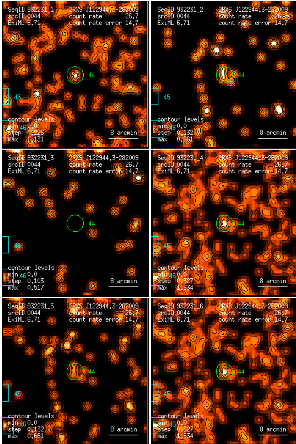
Figure 44: RASS 932231: detection 0044: band rate images, Gaussian filter: (1) PSPC channels 11 – 41, (2) 52 – 90, (3) 91 – 201, (4) 11 – 235, (5) 52 – 201, (6) 11 – 201. Broad band rates in counts/ks. Band rate contour levels in counts/ks/arcmin 2 .
