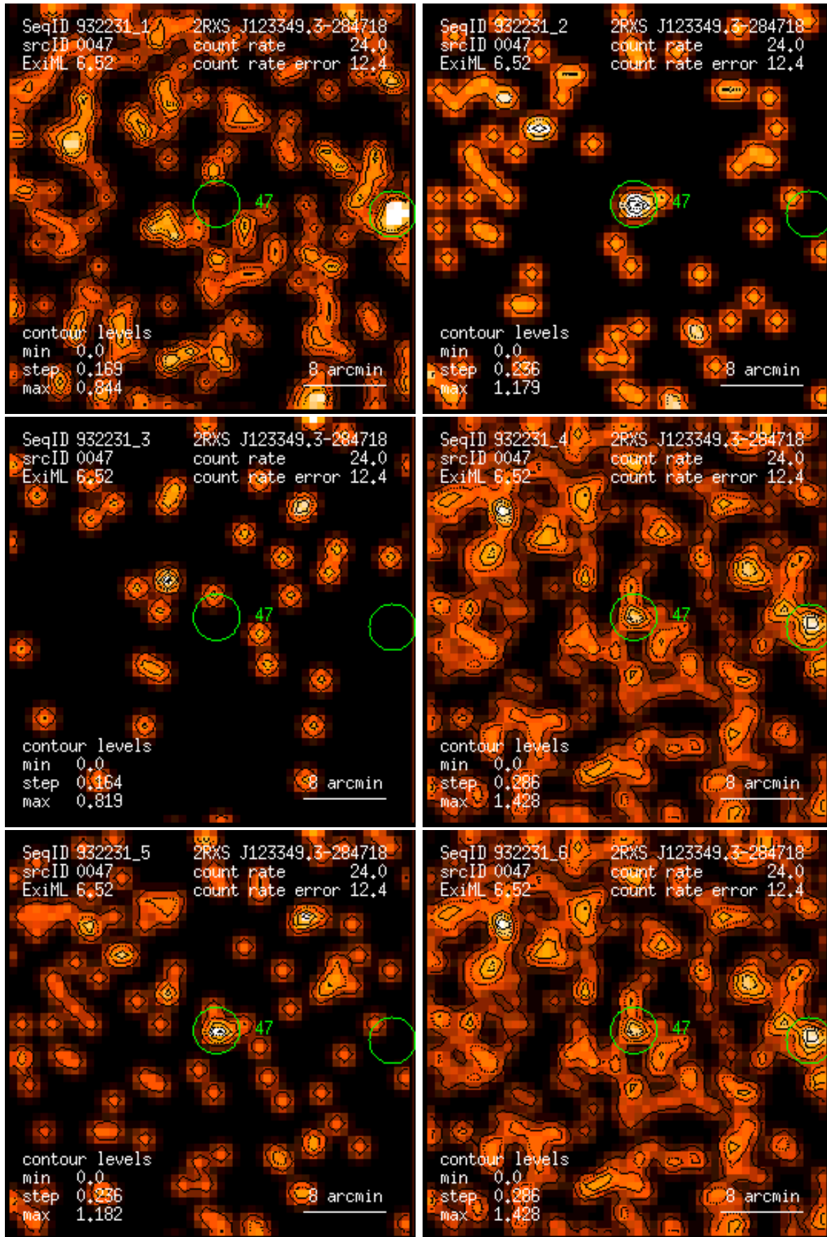
Figure 47: RASS 932231: detection 0047: band rate images, Gaussian filter: (1) PSPC channels 11 – 41, (2) 52 – 90, (3) 91 – 201, (4) 11 – 235, (5) 52 – 201, (6) 11 – 201. Broad band rates in counts/ks. Band rate contour levels in counts/ks/arcmin 2 .
