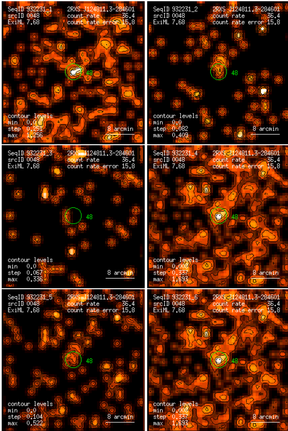
Figure 48: RASS 932231: detection 0048: band rate images, Gaussian filter: (1) PSPC channels 11 – 41, (2) 52 – 90, (3) 91 – 201, (4) 11 – 235, (5) 52 – 201, (6) 11 – 201. Broad band rates in counts/ks. Band rate contour levels in counts/ks/arcmin 2 .
