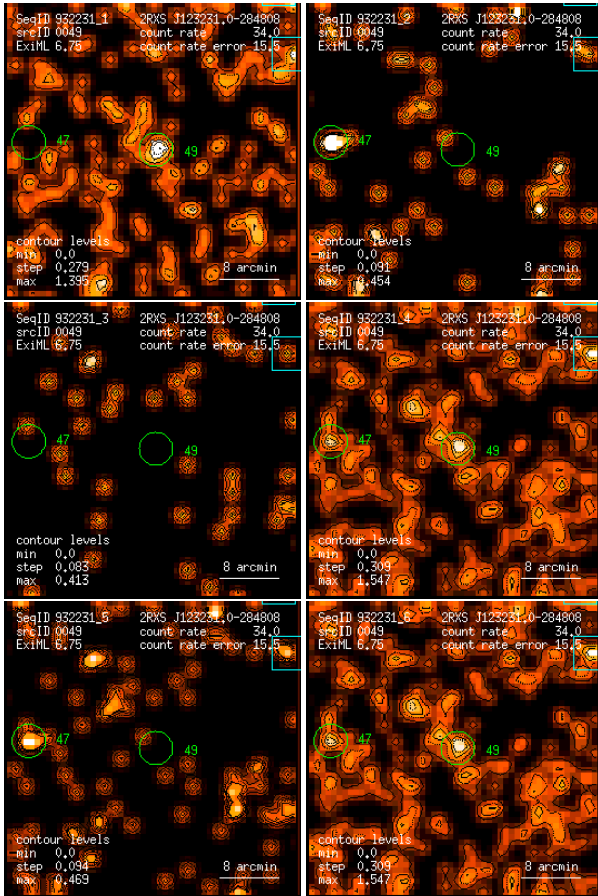
Figure 49: RASS 932231: detection 0049: band rate images, Gaussian filter: (1) PSPC channels 11 – 41, (2) 52 – 90, (3) 91 – 201, (4) 11 – 235, (5) 52 – 201, (6) 11 – 201. Broad band rates in counts/ks. Band rate contour levels in counts/ks/arcmin 2 .
