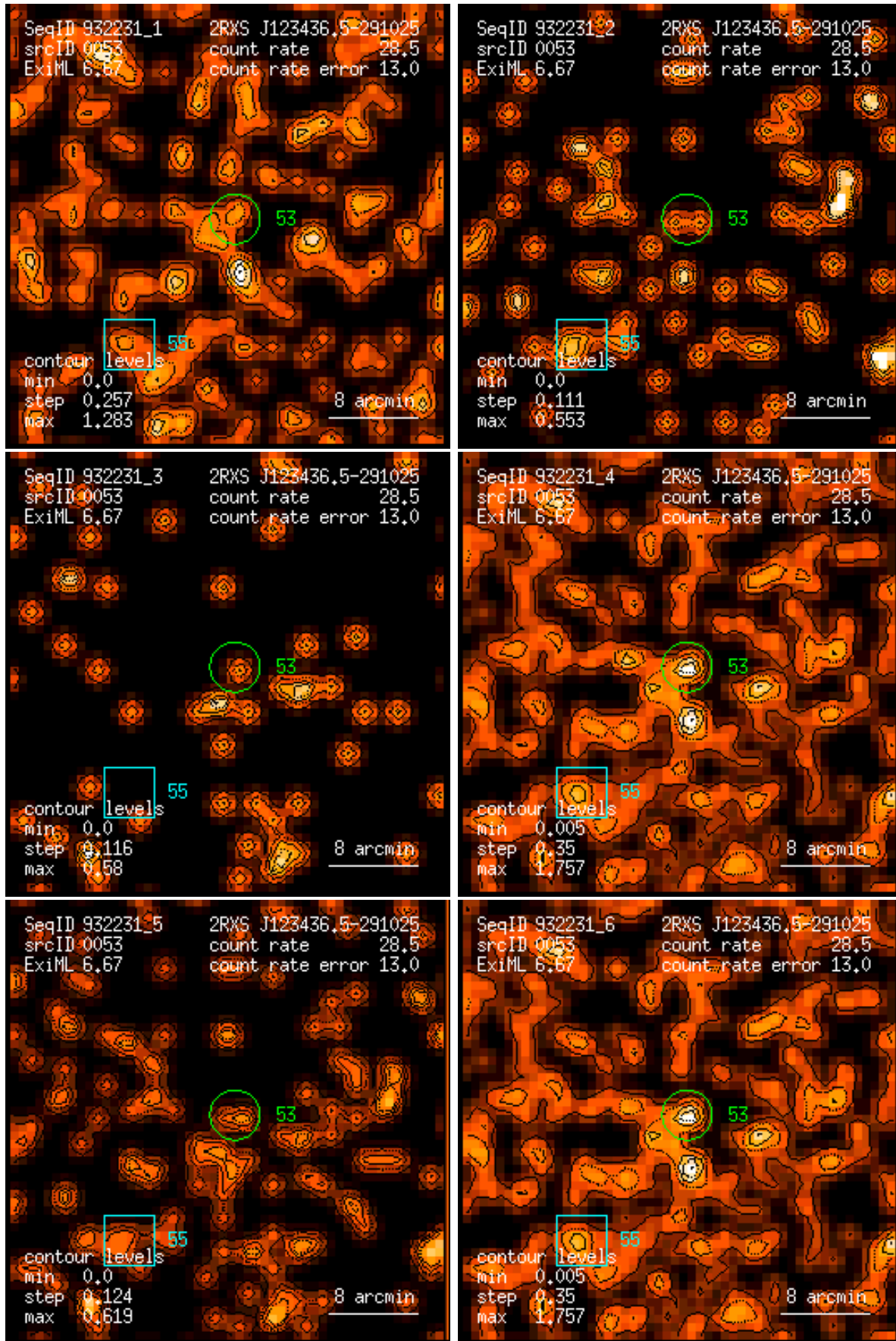
Figure 53: RASS 932231: detection 0053: band rate images, Gaussian filter: (1) PSPC channels 11 – 41, (2) 52 – 90, (3) 91 – 201, (4) 11 – 235, (5) 52 – 201, (6) 11 – 201. Broad band rates in counts/ks. Band rate contour levels in counts/ks/arcmin 2 .
