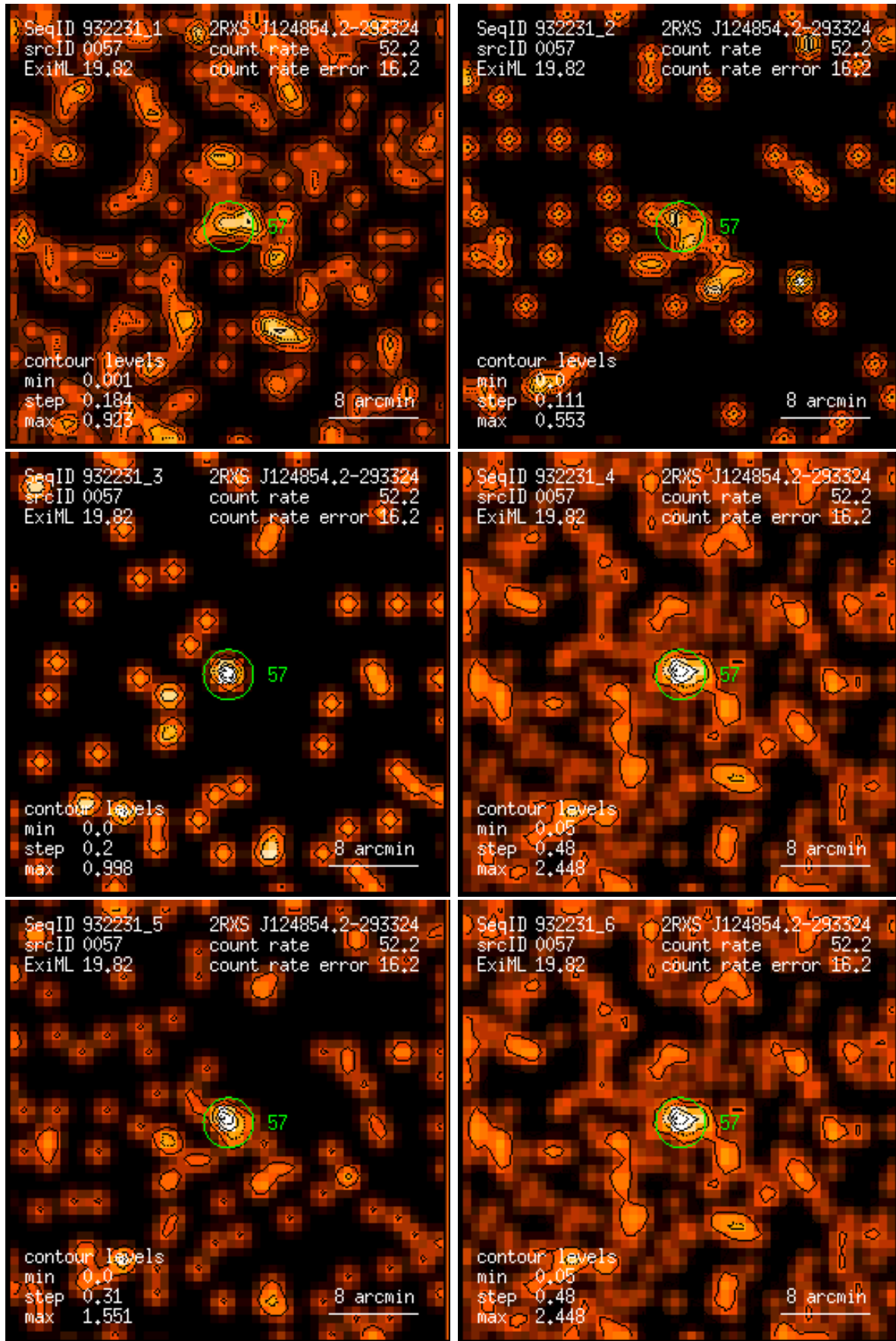
Figure 57: RASS 932231: detection 0057: band rate images, Gaussian filter: (1) PSPC channels 11 – 41, (2) 52 – 90, (3) 91 – 201, (4) 11 – 235, (5) 52 – 201, (6) 11 – 201. Broad band rates in counts/ks. Band rate contour levels in counts/ks/arcmin 2 .
